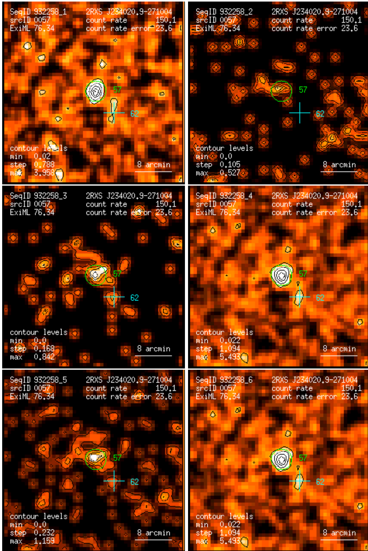
Figure 57: RASS 932258: detection 0057: band rate images, Gaussian filter: (1) PSPC channels 11 – 41, (2) 52 – 90, (3) 91 – 201, (4) 11 – 235, (5) 52 – 201, (6) 11 – 201. Broad band rates in counts/ks. Band rate contour levels in counts/ks/arcmin 2 .
