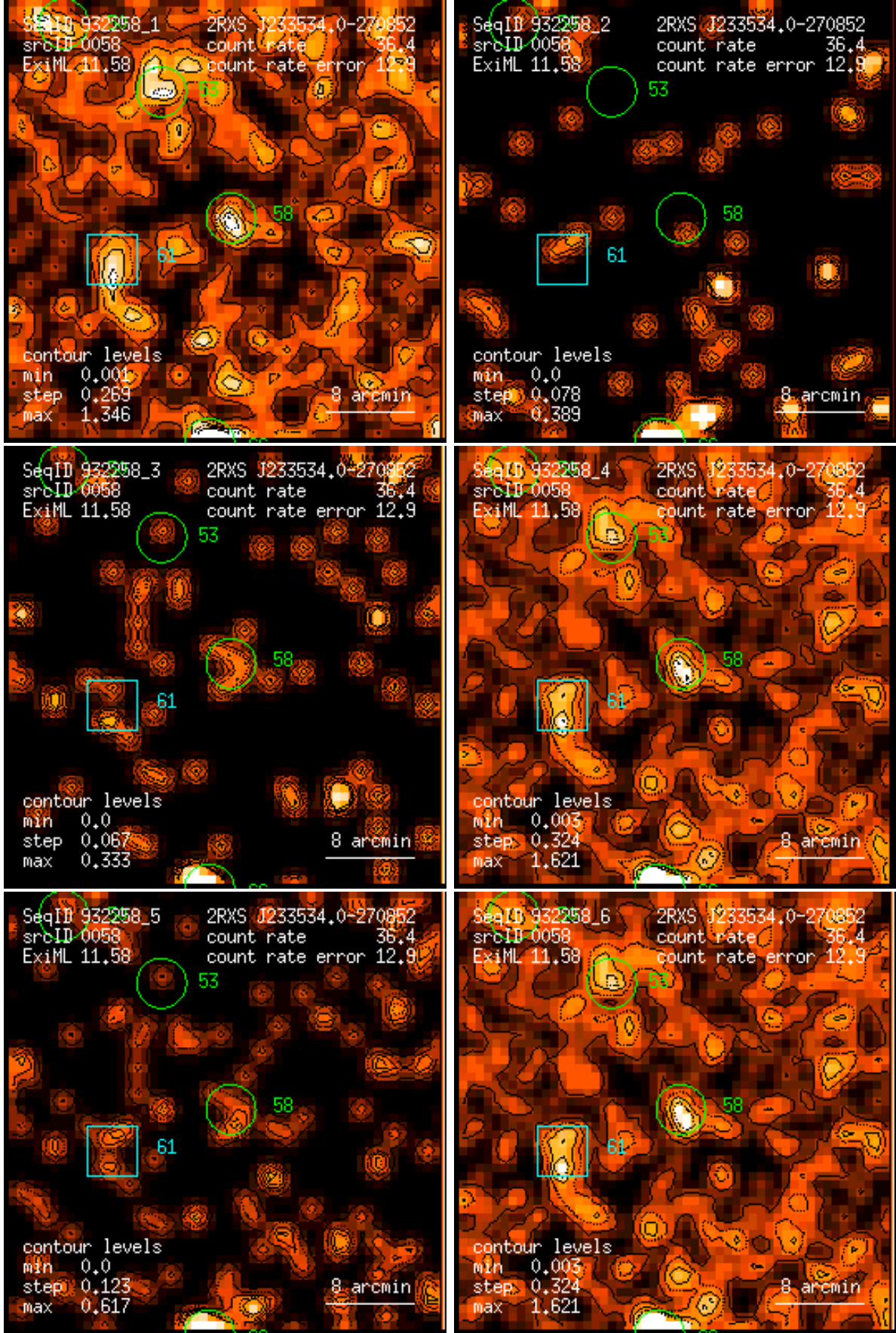
Figure 58: RASS 932258: detection 0058: band rate images, Gaussian filter: (1) PSPC channels 11 – 41, (2) 52 – 90, (3) 91 – 201, (4) 11 – 235, (5) 52 – 201, (6) 11 – 201. Broad band rates in counts/ks. Band rate contour levels in counts/ks/arcmin 2 .
