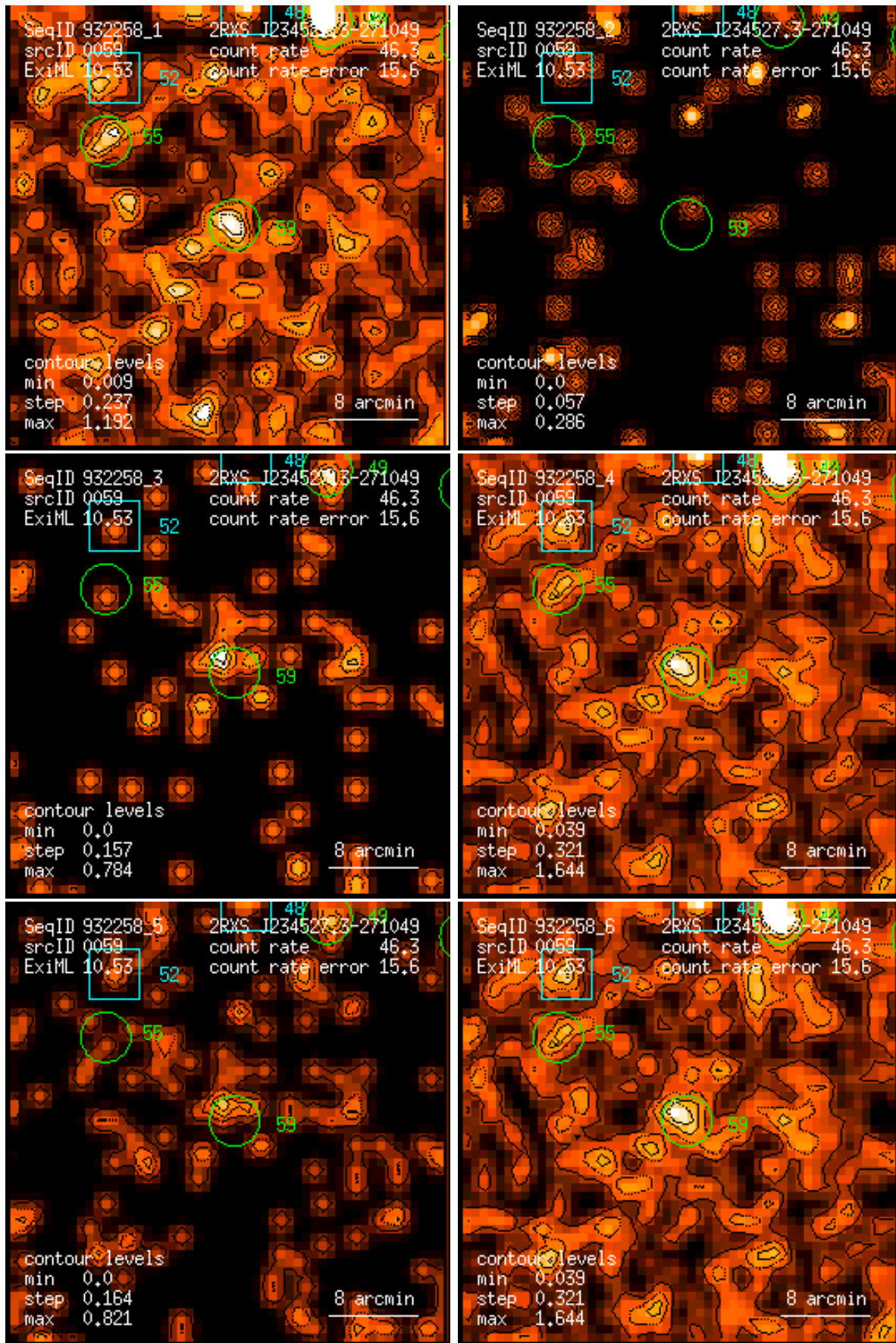
Figure 59: RASS 932258: detection 0059: band rate images, Gaussian filter: (1) PSPC channels 11 – 41, (2) 52 – 90, (3) 91 – 201, (4) 11 – 235, (5) 52 – 201, (6) 11 – 201. Broad band rates in counts/ks. Band rate contour levels in counts/ks/arcmin 2 .
