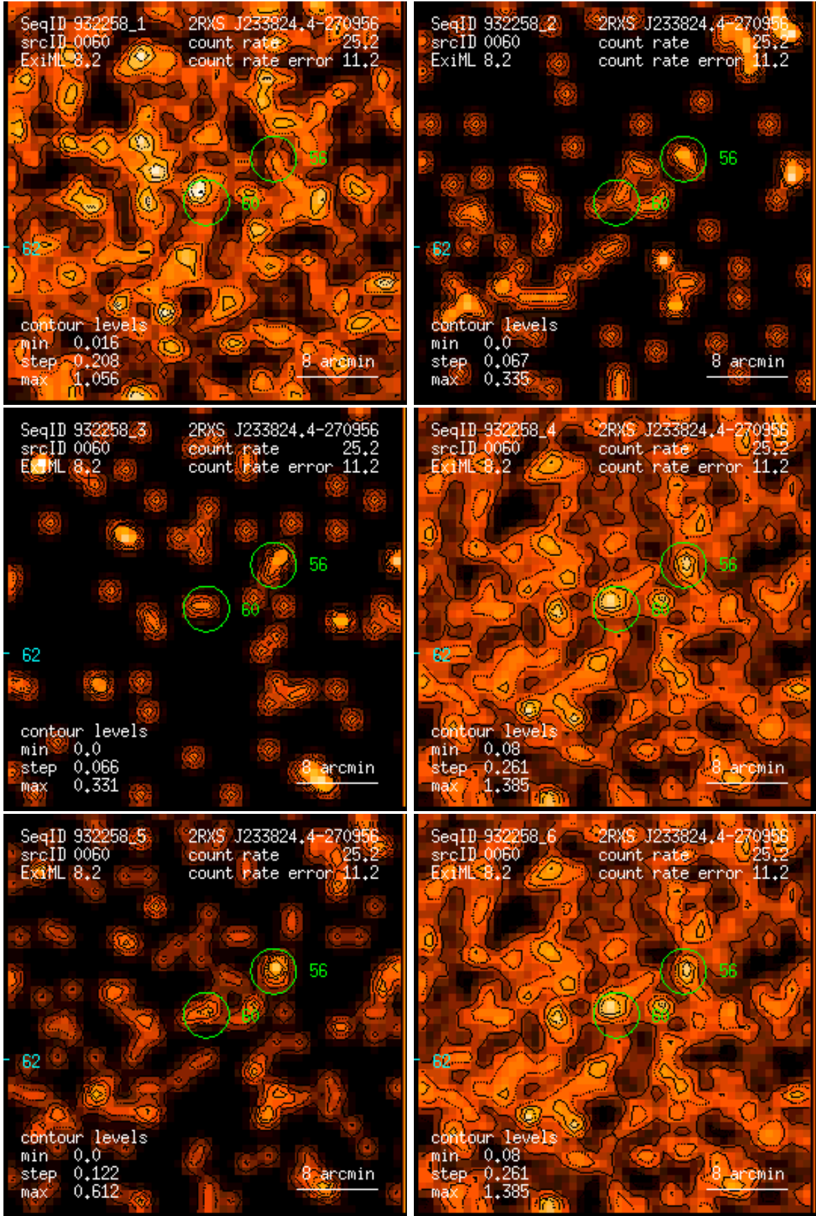
Figure 60: RASS 932258: detection 0060: band rate images, Gaussian filter: (1) PSPC channels 11 – 41, (2) 52 – 90, (3) 91 – 201, (4) 11 – 235, (5) 52 – 201, (6) 11 – 201. Broad band rates in counts/ks. Band rate contour levels in counts/ks/arcmin 2 .
