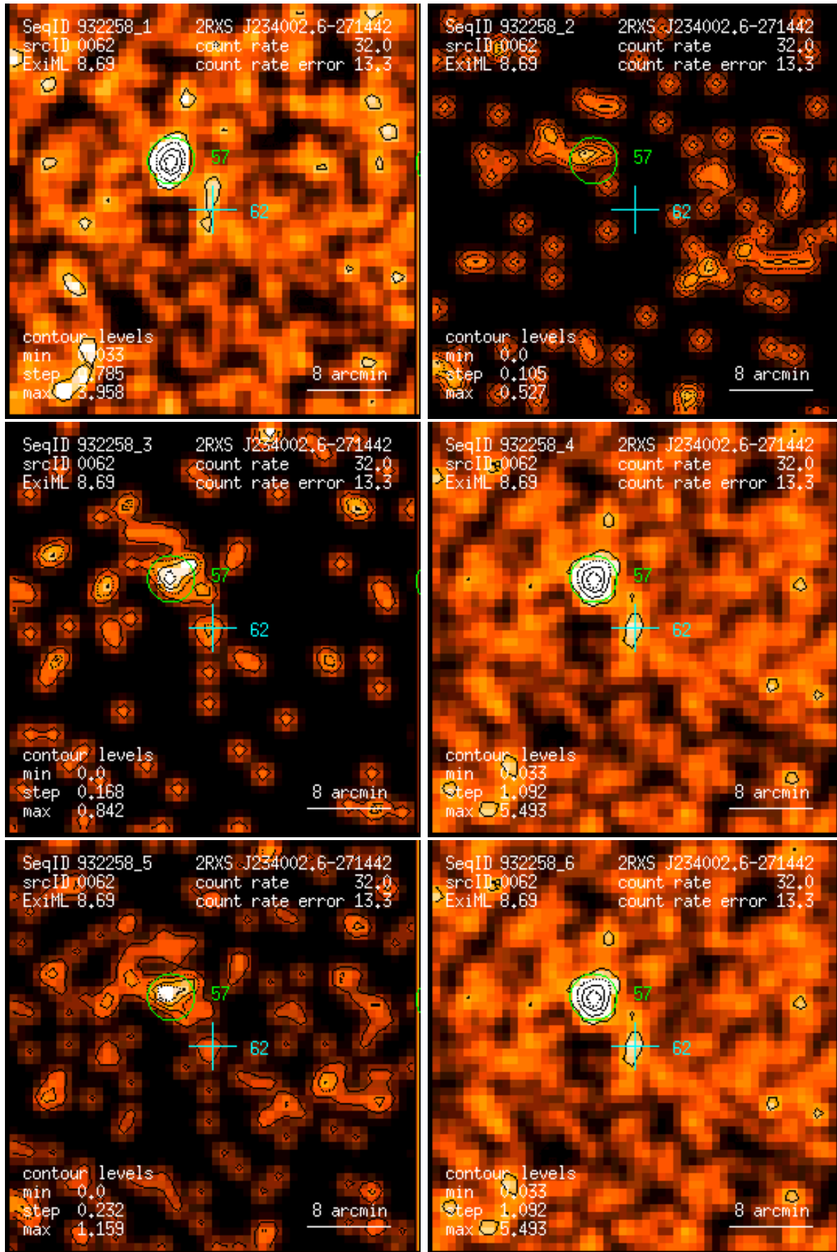
Figure 62: RASS 932258: detection 0062: band rate images, Gaussian filter: (1) PSPC channels 11 – 41, (2) 52 – 90, (3) 91 – 201, (4) 11 – 235, (5) 52 – 201, (6) 11 – 201. Broad band rates in counts/ks. Band rate contour levels in counts/ks/arcmin 2 .
