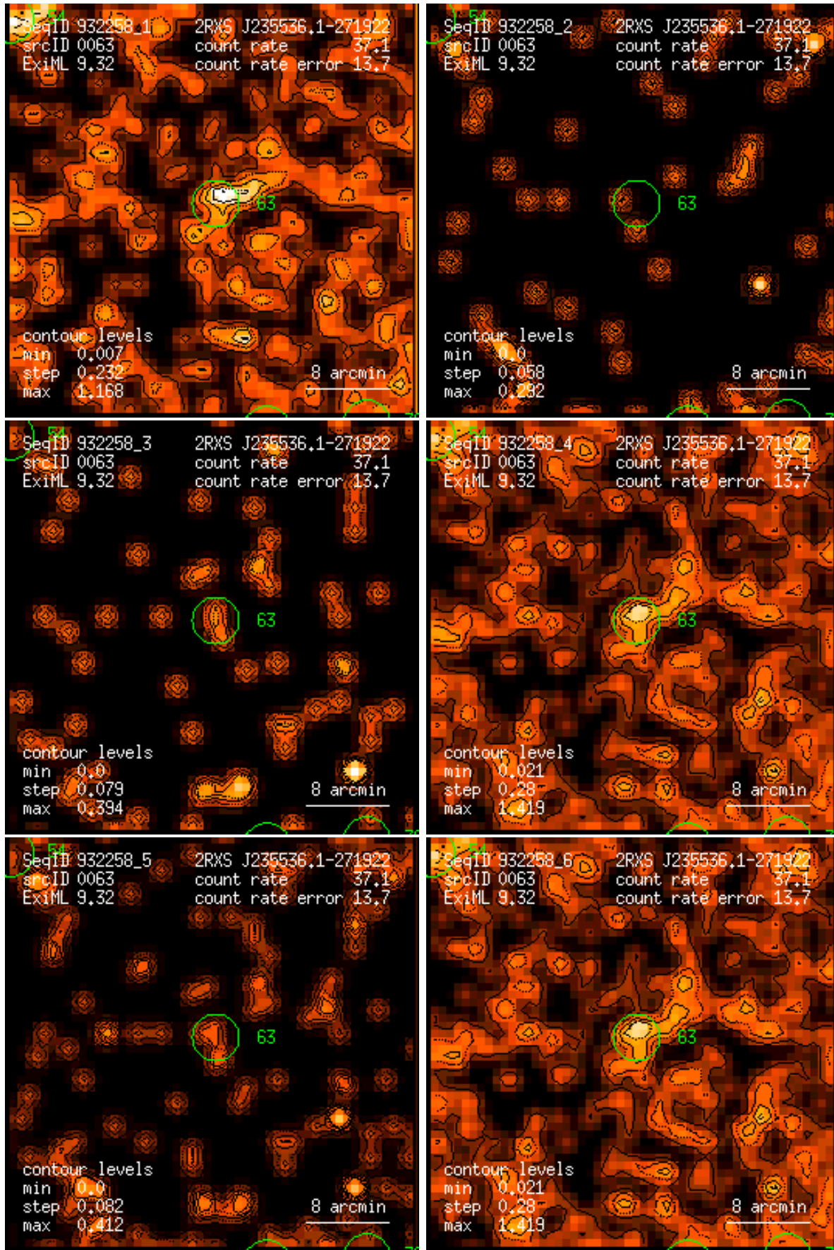
Figure 63: RASS 932258: detection 0063: band rate images, Gaussian filter: (1) PSPC channels 11 – 41, (2) 52 – 90, (3) 91 – 201, (4) 11 – 235, (5) 52 – 201, (6) 11 – 201. Broad band rates in counts/ks. Band rate contour levels in counts/ks/arcmin 2 .
