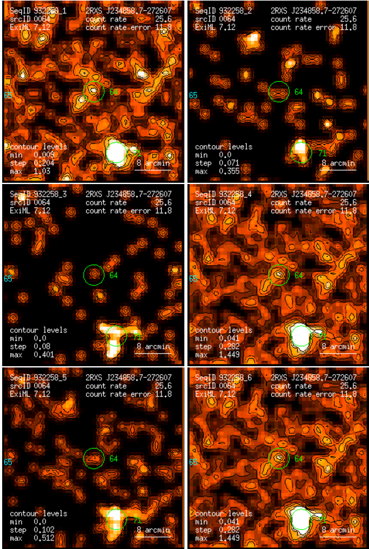
Figure 64: RASS 932258: detection 0064: band rate images, Gaussian filter: (1) PSPC channels 11 – 41, (2) 52 – 90, (3) 91 – 201, (4) 11 – 235, (5) 52 – 201, (6) 11 – 201. Broad band rates in counts/ks. Band rate contour levels in counts/ks/arcmin 2 .
