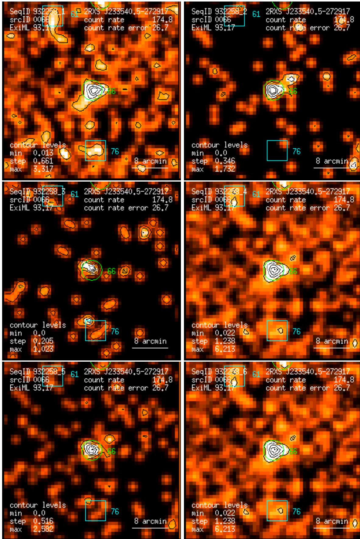
Figure 66: RASS 932258: detection 0066: band rate images, Gaussian filter: (1) PSPC channels 11 – 41, (2) 52 – 90, (3) 91 – 201, (4) 11 – 235, (5) 52 – 201, (6) 11 – 201. Broad band rates in counts/ks. Band rate contour levels in counts/ks/arcmin 2 .
