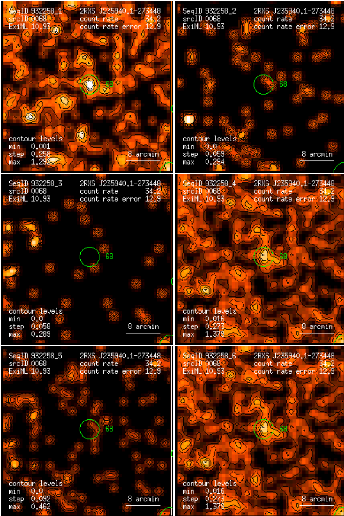
Figure 68: RASS 932258: detection 0068: band rate images, Gaussian filter: (1) PSPC channels 11 – 41, (2) 52 – 90, (3) 91 – 201, (4) 11 – 235, (5) 52 – 201, (6) 11 – 201. Broad band rates in counts/ks. Band rate contour levels in counts/ks/arcmin 2 .
