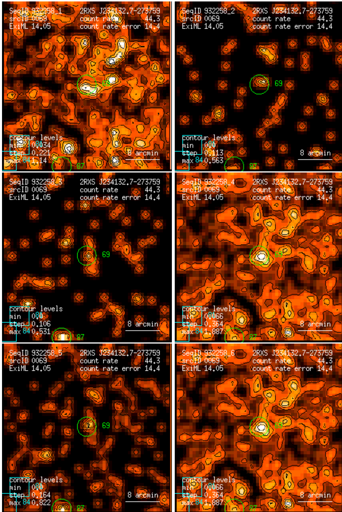
Figure 69: RASS 932258: detection 0069: band rate images, Gaussian filter: (1) PSPC channels 11 – 41, (2) 52 – 90, (3) 91 – 201, (4) 11 – 235, (5) 52 – 201, (6) 11 – 201. Broad band rates in counts/ks. Band rate contour levels in counts/ks/arcmin 2 .
