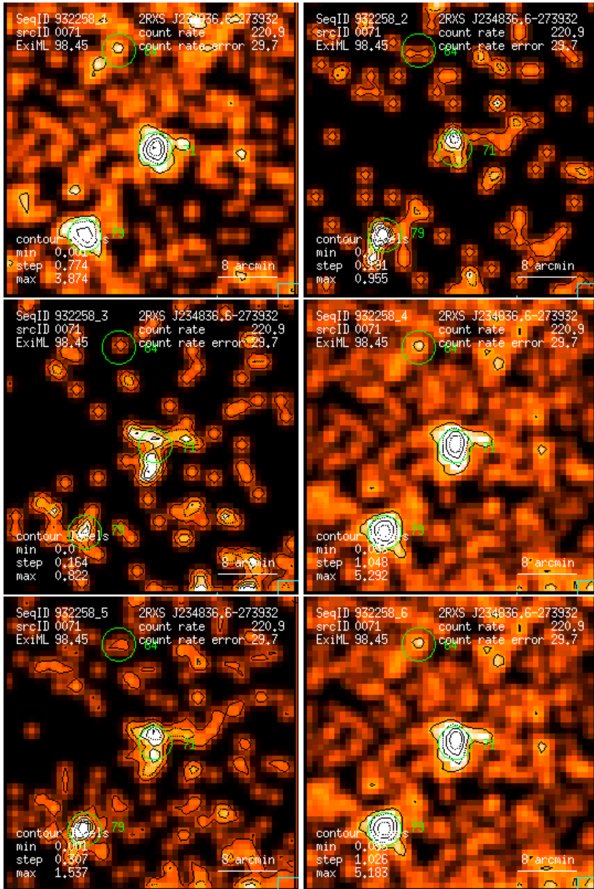
Figure 71: RASS 932258: detection 0071: band rate images, Gaussian filter: (1) PSPC channels 11 – 41, (2) 52 – 90, (3) 91 – 201, (4) 11 – 235, (5) 52 – 201, (6) 11 – 201. Broad band rates in counts/ks. Band rate contour levels in counts/ks/arcmin 2 .
