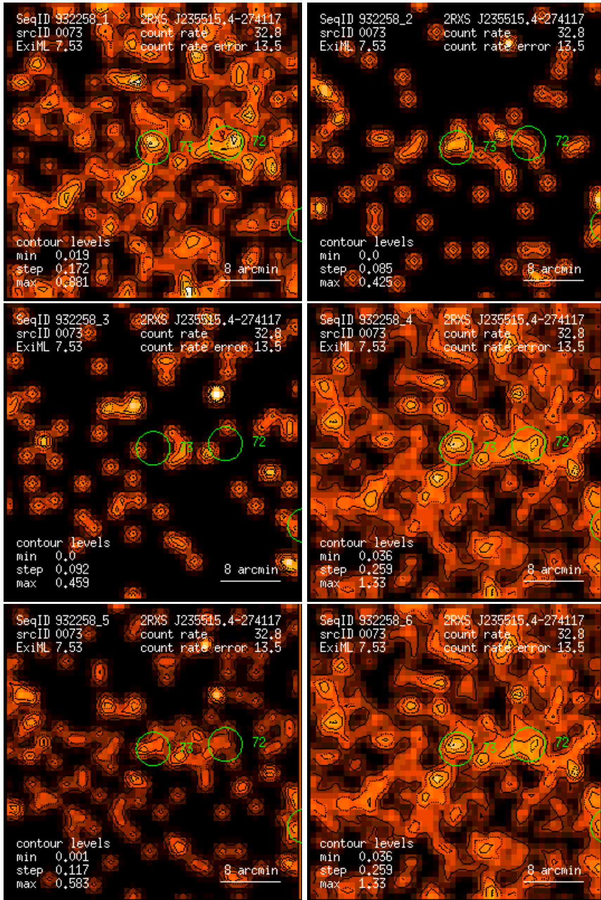
Figure 73: RASS 932258: detection 0073: band rate images, Gaussian filter: (1) PSPC channels 11 – 41, (2) 52 – 90, (3) 91 – 201, (4) 11 – 235, (5) 52 – 201, (6) 11 – 201. Broad band rates in counts/ks. Band rate contour levels in counts/ks/arcmin 2 .
