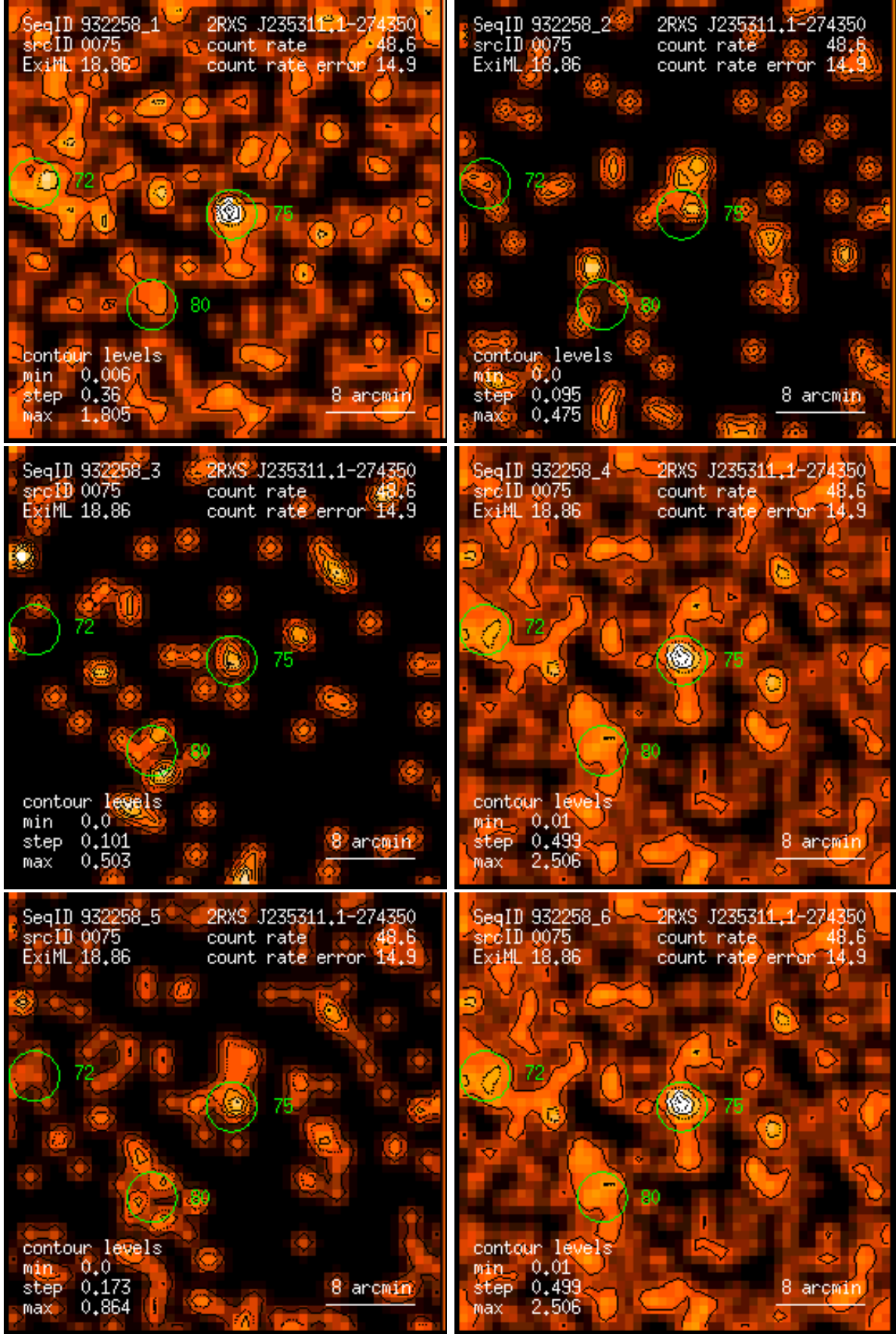
Figure 75: RASS 932258: detection 0075: band rate images, Gaussian filter: (1) PSPC channels 11 – 41, (2) 52 – 90, (3) 91 – 201, (4) 11 – 235, (5) 52 – 201, (6) 11 – 201. Broad band rates in counts/ks. Band rate contour levels in counts/ks/arcmin 2 .
