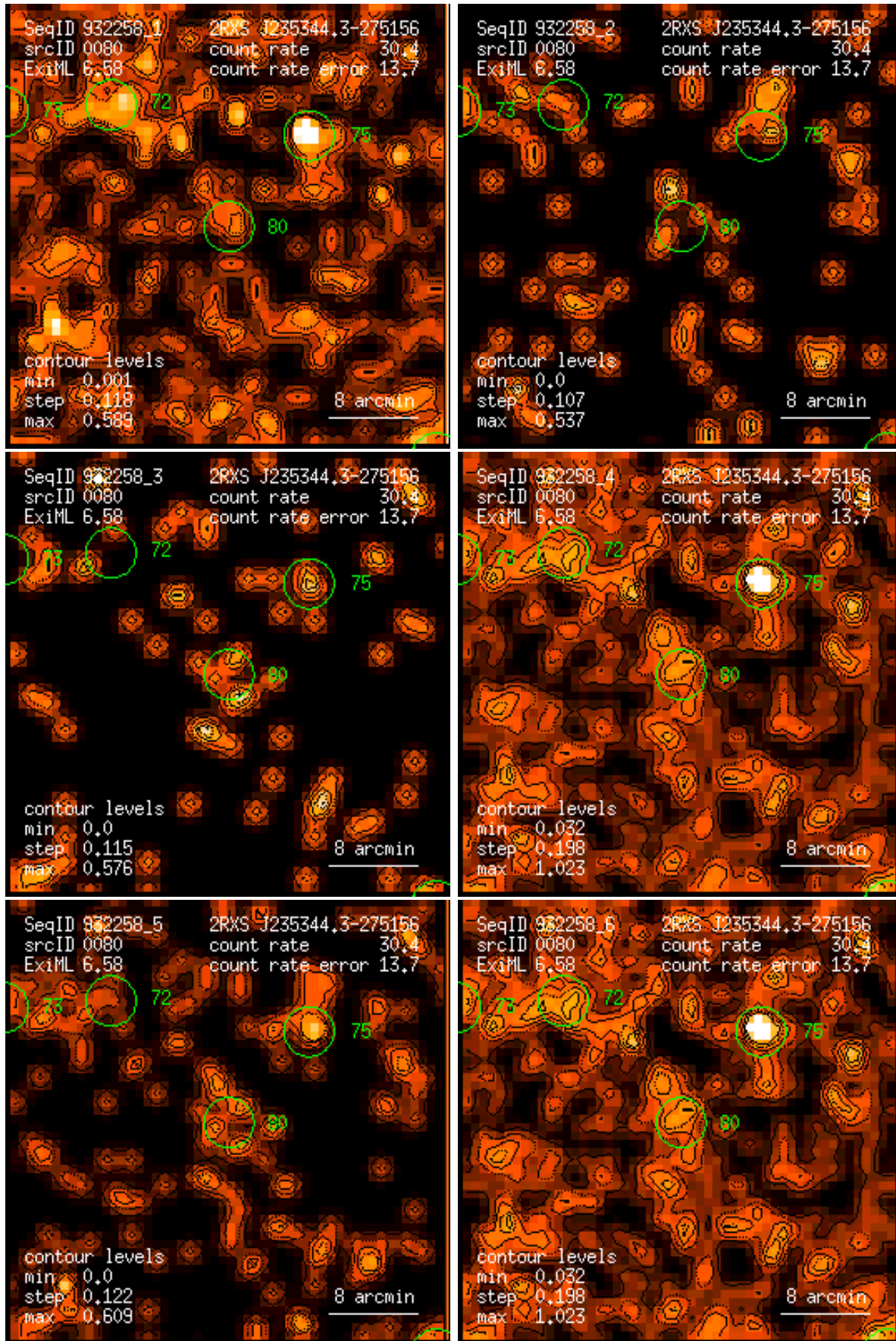
Figure 80: RASS 932258: detection 0080: band rate images, Gaussian filter: (1) PSPC channels 11 – 41, (2) 52 – 90, (3) 91 – 201, (4) 11 – 235, (5) 52 – 201, (6) 11 – 201. Broad band rates in counts/ks. Band rate contour levels in counts/ks/arcmin 2 .
