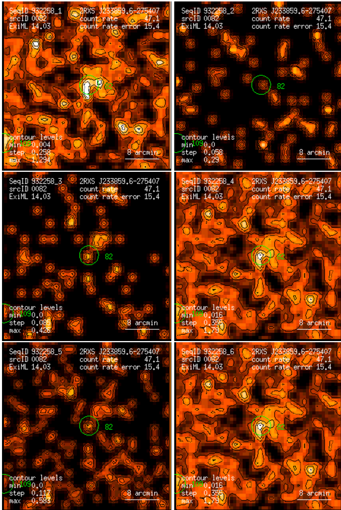
Figure 82: RASS 932258: detection 0082: band rate images, Gaussian filter: (1) PSPC channels 11 – 41, (2) 52 – 90, (3) 91 – 201, (4) 11 – 235, (5) 52 – 201, (6) 11 – 201. Broad band rates in counts/ks. Band rate contour levels in counts/ks/arcmin 2 .
