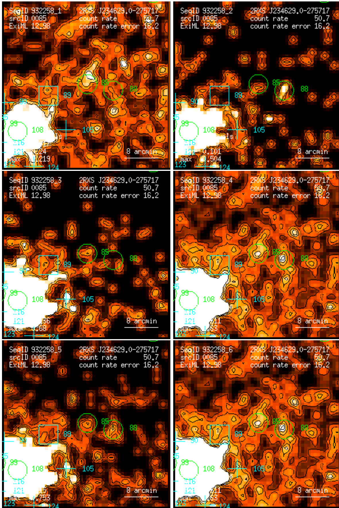
Figure 85: RASS 932258: detection 0085: band rate images, Gaussian filter: (1) PSPC channels 11 – 41, (2) 52 – 90, (3) 91 – 201, (4) 11 – 235, (5) 52 – 201, (6) 11 – 201. Broad band rates in counts/ks. Band rate contour levels in counts/ks/arcmin 2 .
