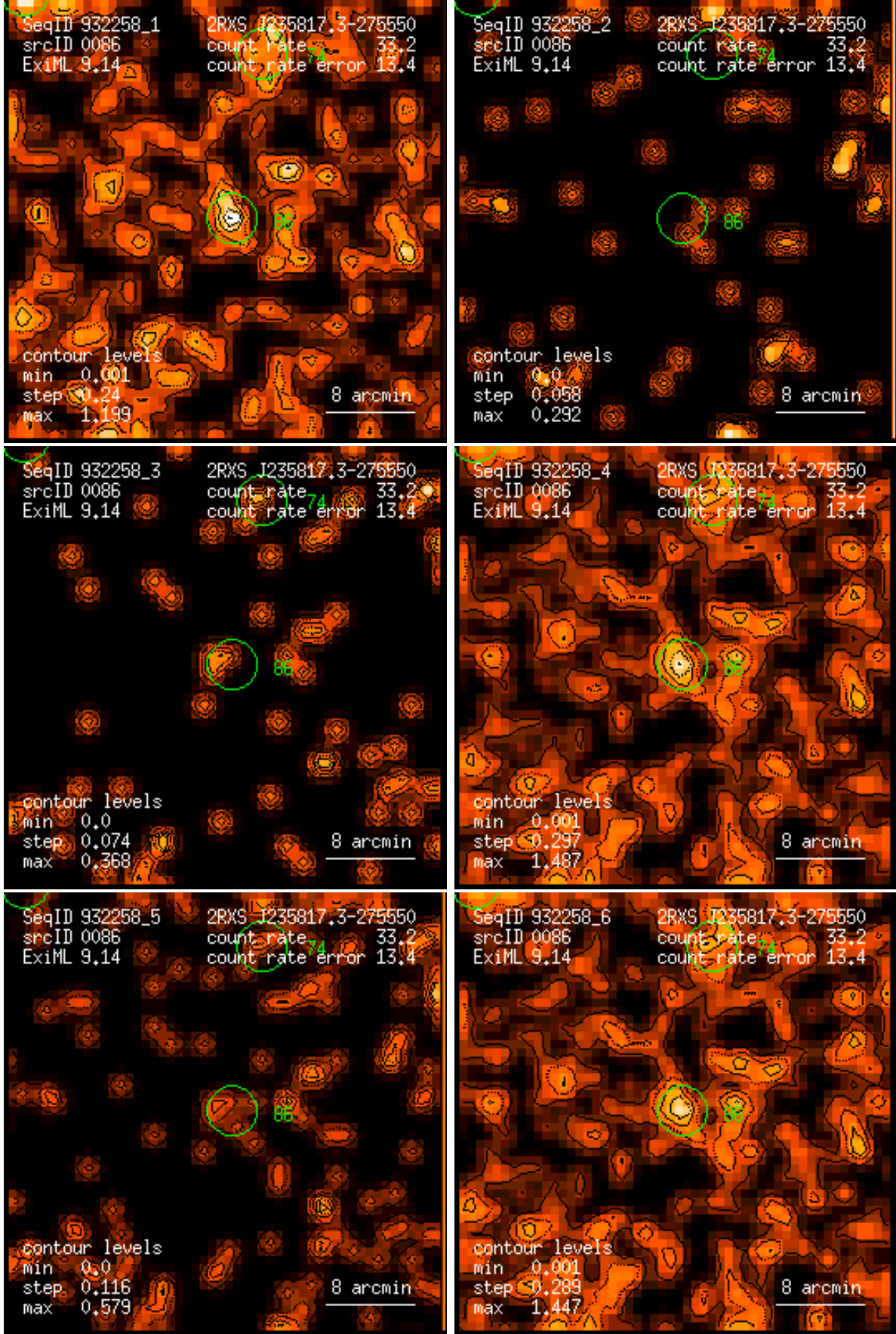
Figure 86: RASS 932258: detection 0086: band rate images, Gaussian filter: (1) PSPC channels 11 – 41, (2) 52 – 90, (3) 91 – 201, (4) 11 – 235, (5) 52 – 201, (6) 11 – 201. Broad band rates in counts/ks. Band rate contour levels in counts/ks/arcmin 2 .
