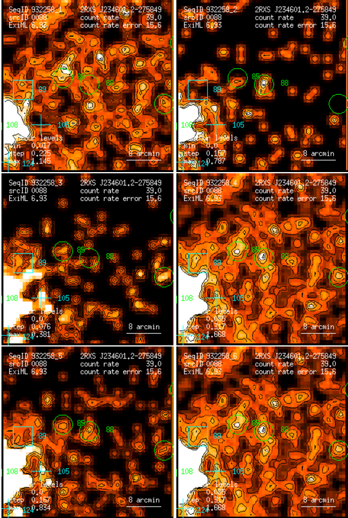
Figure 88: RASS 932258: detection 0088: band rate images, Gaussian filter: (1) PSPC channels 11 – 41, (2) 52 – 90, (3) 91 – 201, (4) 11 – 235, (5) 52 – 201, (6) 11 – 201. Broad band rates in counts/ks. Band rate contour levels in counts/ks/arcmin 2 .
