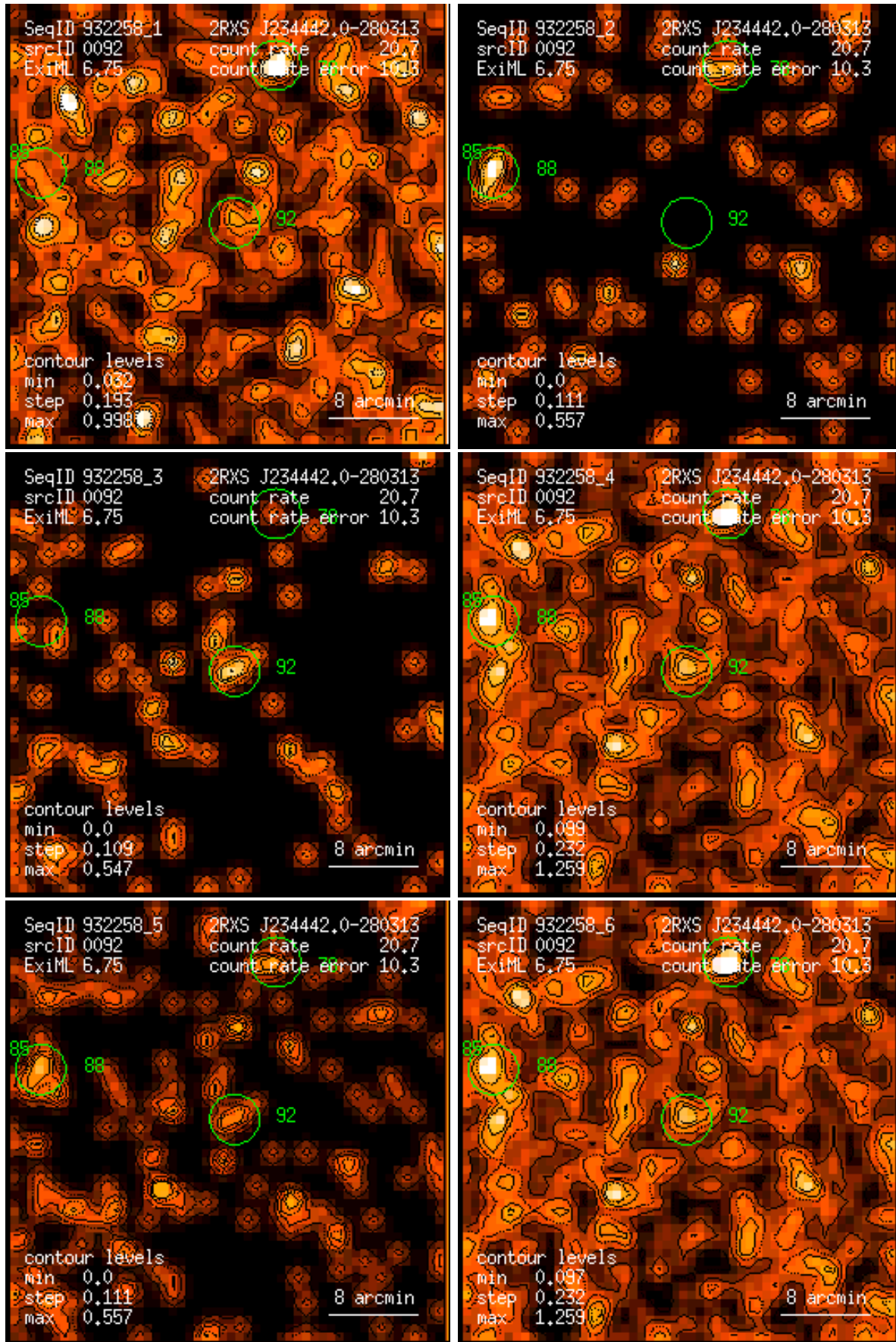
Figure 92: RASS 932258: detection 0092: band rate images, Gaussian filter: (1) PSPC channels 11 – 41, (2) 52 – 90, (3) 91 – 201, (4) 11 – 235, (5) 52 – 201, (6) 11 – 201. Broad band rates in counts/ks. Band rate contour levels in counts/ks/arcmin 2 .
