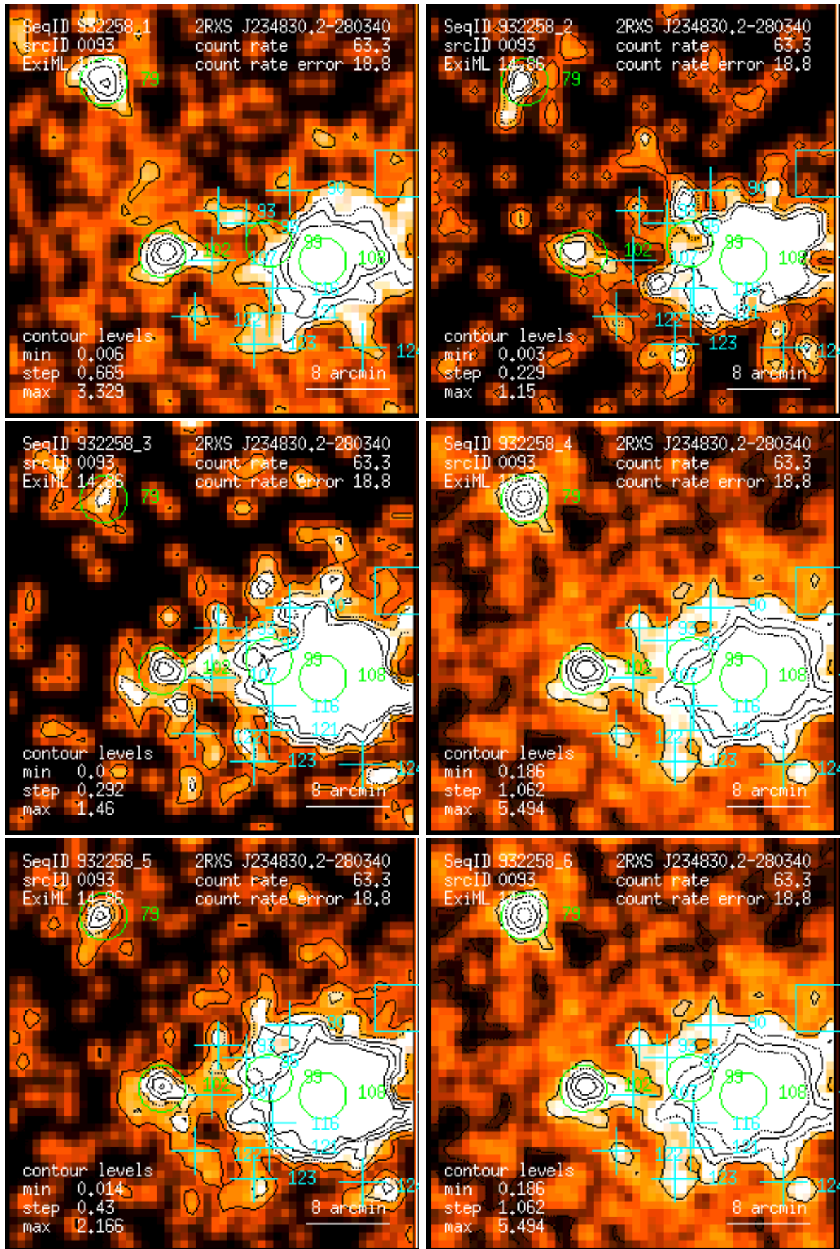
Figure 93: RASS 932258: detection 0093: band rate images, Gaussian filter: (1) PSPC channels 11 – 41, (2) 52 – 90, (3) 91 – 201, (4) 11 – 235, (5) 52 – 201, (6) 11 – 201. Broad band rates in counts/ks. Band rate contour levels in counts/ks/arcmin 2 .
