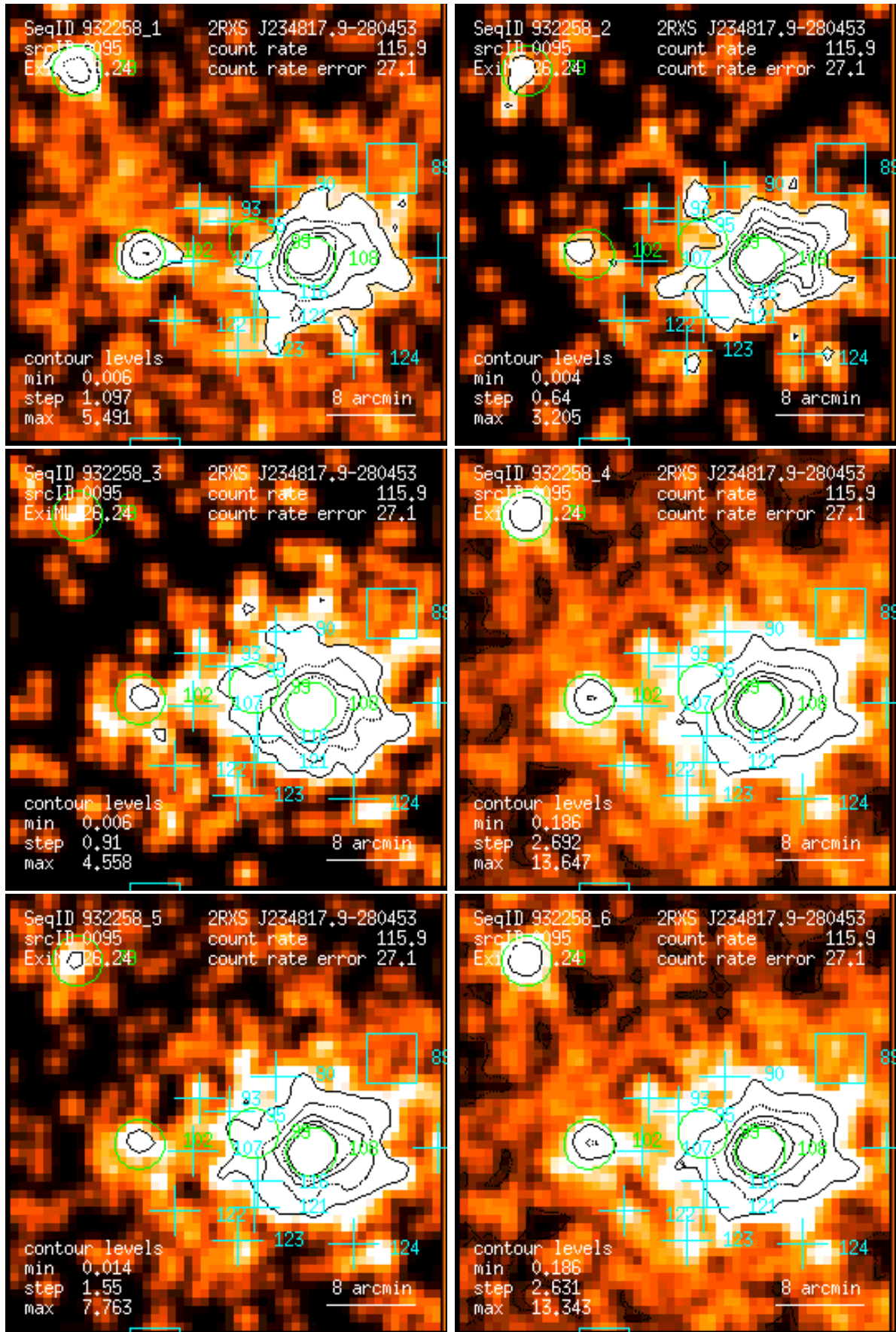
Figure 95: RASS 932258: detection 0095: band rate images, Gaussian filter: (1) PSPC channels 11 – 41, (2) 52 – 90, (3) 91 – 201, (4) 11 – 235, (5) 52 – 201, (6) 11 – 201. Broad band rates in counts/ks. Band rate contour levels in counts/ks/arcmin 2 .
