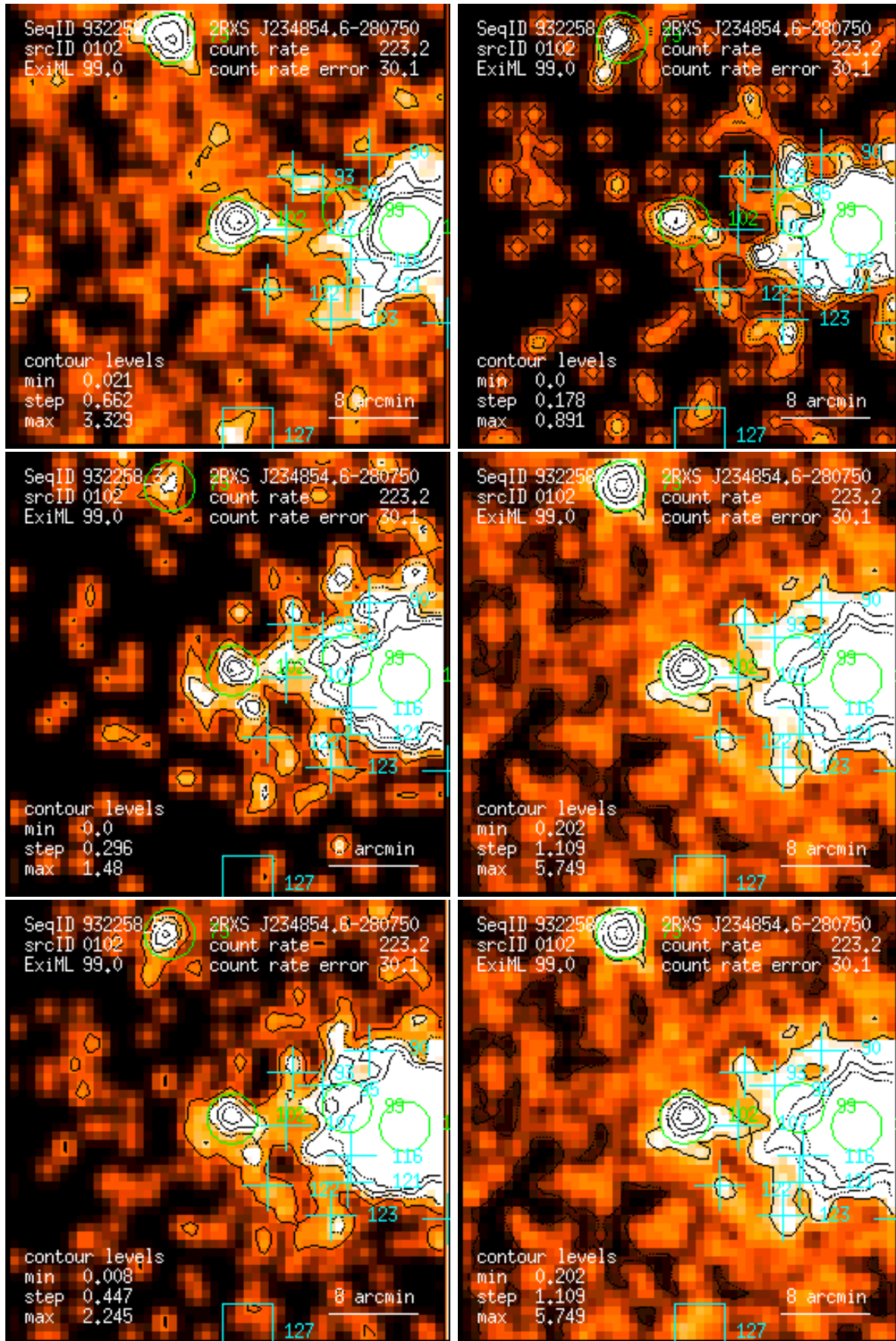
Figure 102: RASS 932258: detection 0102: band rate images, Gaussian filter: (1) PSPC channels 11 – 41, (2) 52 – 90, (3) 91 – 201, (4) 11 – 235, (5) 52 – 201, (6) 11 – 201. Broad band rates in counts/ks. Band rate contour levels in counts/ks/arcmin 2 .
