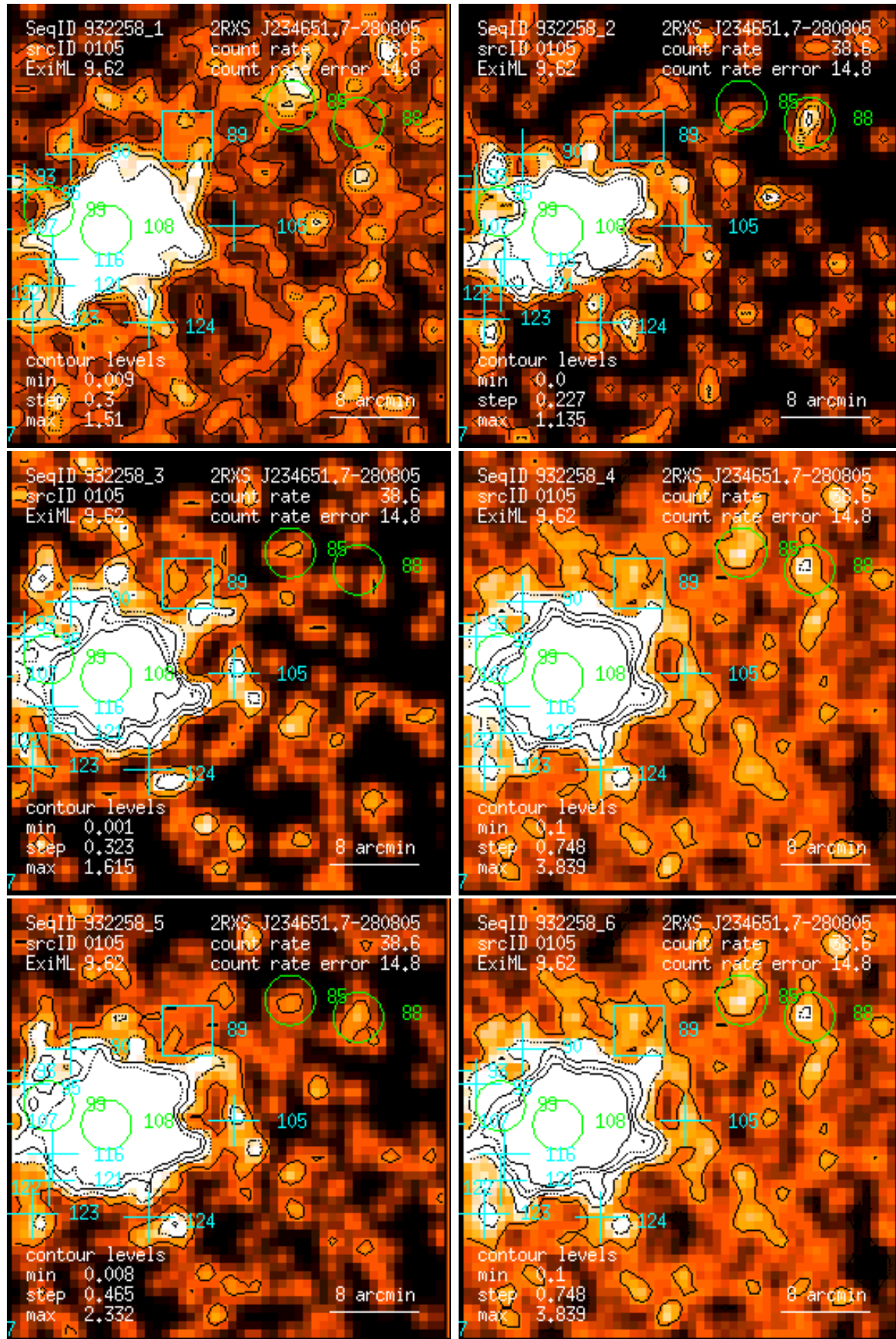
Figure 105: RASS 932258: detection 0105: band rate images, Gaussian filter: (1) PSPC channels 11 – 41, (2) 52 – 90, (3) 91 – 201, (4) 11 – 235, (5) 52 – 201, (6) 11 – 201. Broad band rates in counts/ks. Band rate contour levels in counts/ks/arcmin 2 .
