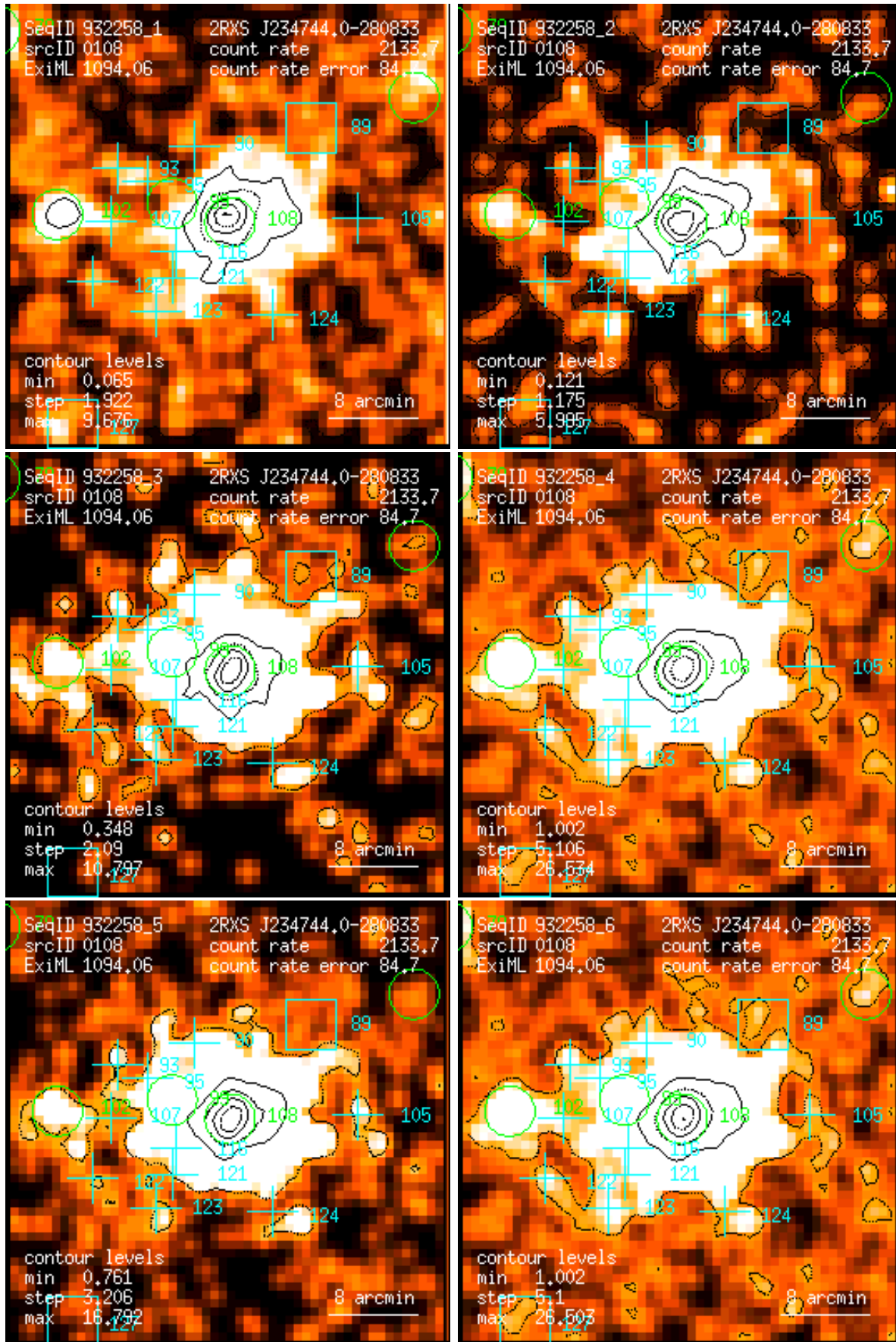
Figure 108: RASS 932258: detection 0108: band rate images, Gaussian filter: (1) PSPC channels 11 – 41, (2) 52 – 90, (3) 91 – 201, (4) 11 – 235, (5) 52 – 201, (6) 11 – 201. Broad band rates in counts/ks. Band rate contour levels in counts/ks/arcmin 2 .
