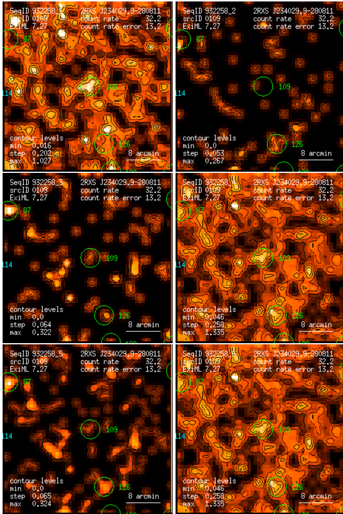
Figure 109: RASS 932258: detection 0109: band rate images, Gaussian filter: (1) PSPC channels 11 – 41, (2) 52 – 90, (3) 91 – 201, (4) 11 – 235, (5) 52 – 201, (6) 11 – 201. Broad band rates in counts/ks. Band rate contour levels in counts/ks/arcmin 2 .
