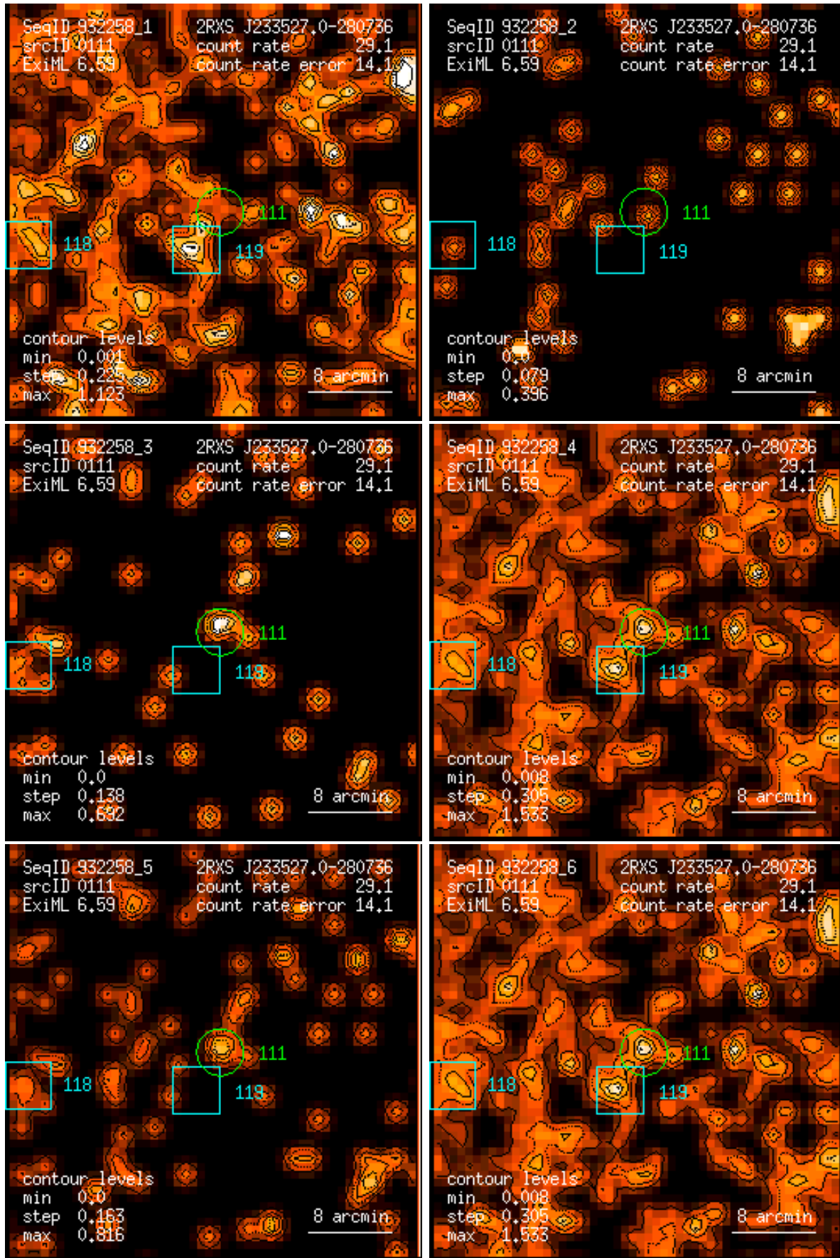
Figure 111: RASS 932258: detection 0111: band rate images, Gaussian filter: (1) PSPC channels 11 – 41, (2) 52 – 90, (3) 91 – 201, (4) 11 – 235, (5) 52 – 201, (6) 11 – 201. Broad band rates in counts/ks. Band rate contour levels in counts/ks/arcmin 2 .
