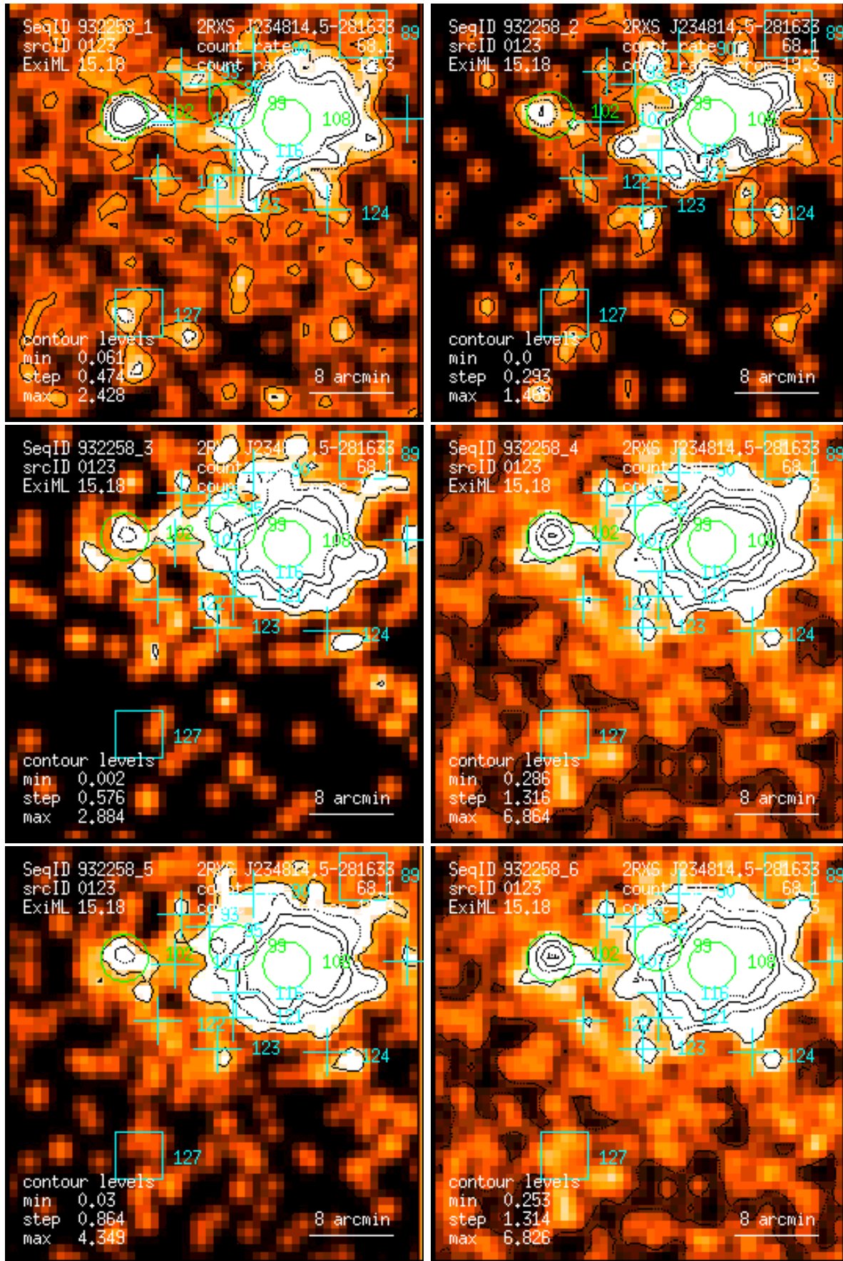
Figure 123: RASS 932258: detection 0123: band rate images, Gaussian filter: (1) PSPC channels 11 – 41, (2) 52 – 90, (3) 91 – 201, (4) 11 – 235, (5) 52 – 201, (6) 11 – 201. Broad band rates in counts/ks. Band rate contour levels in counts/ks/arcmin 2 .
