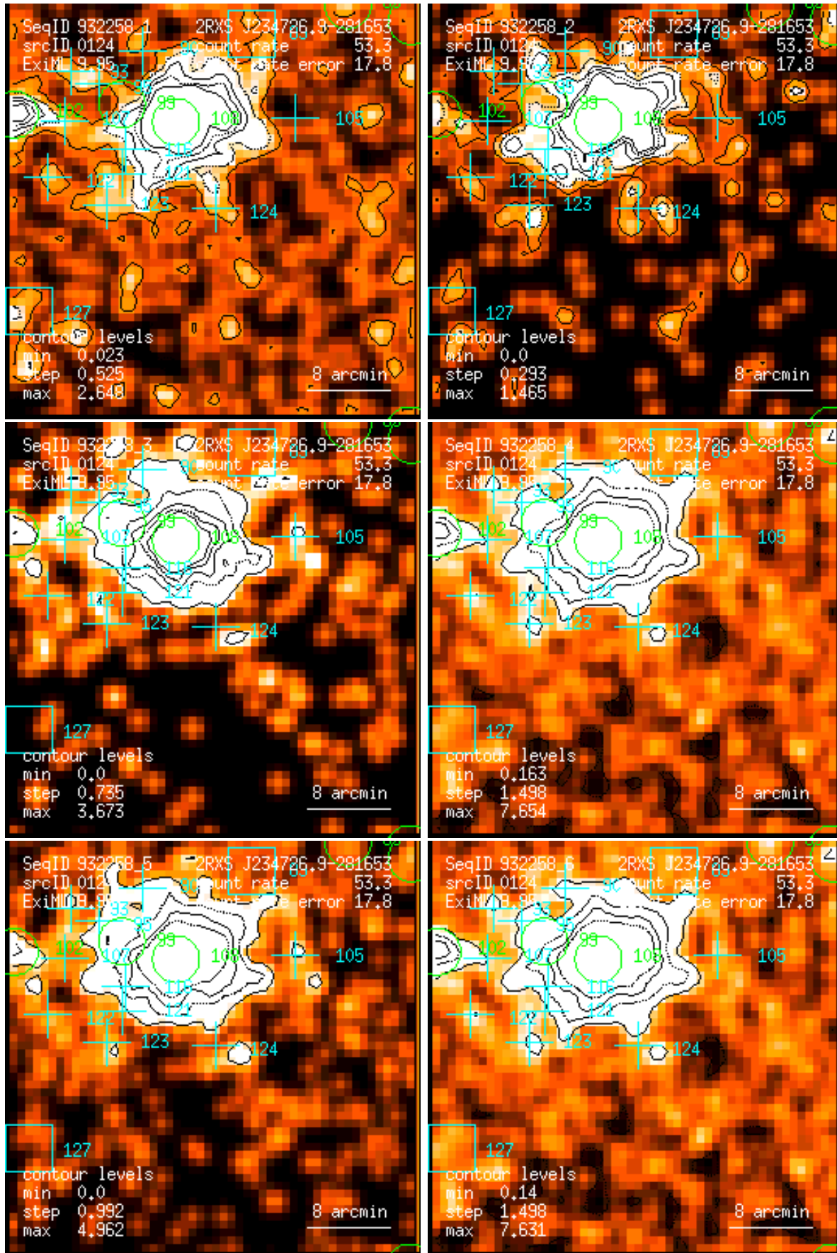
Figure 124: RASS 932258: detection 0124: band rate images, Gaussian filter: (1) PSPC channels 11 – 41, (2) 52 – 90, (3) 91 – 201, (4) 11 – 235, (5) 52 – 201, (6) 11 – 201. Broad band rates in counts/ks. Band rate contour levels in counts/ks/arcmin 2 .
