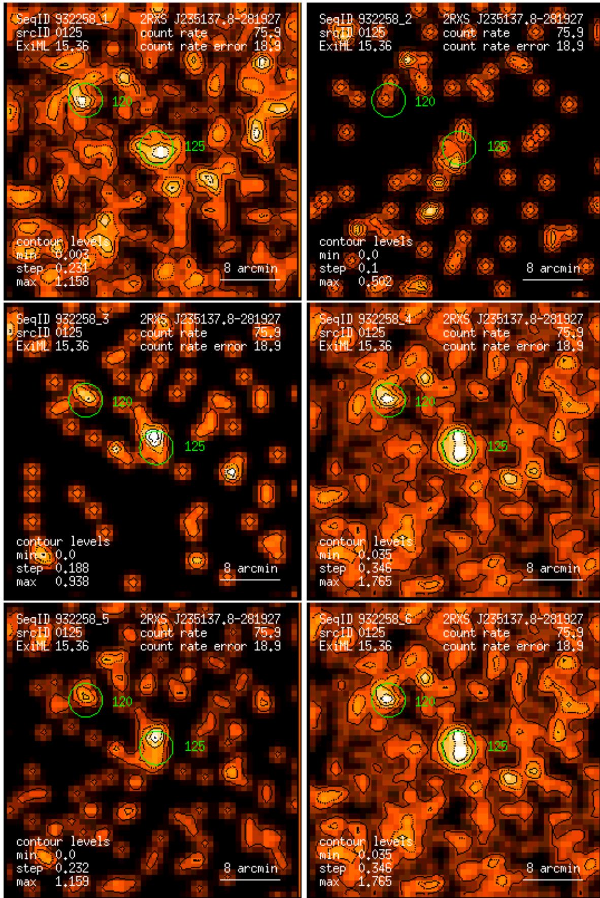
Figure 125: RASS 932258: detection 0125: band rate images, Gaussian filter: (1) PSPC channels 11 – 41, (2) 52 – 90, (3) 91 – 201, (4) 11 – 235, (5) 52 – 201, (6) 11 – 201. Broad band rates in counts/ks. Band rate contour levels in counts/ks/arcmin 2 .
