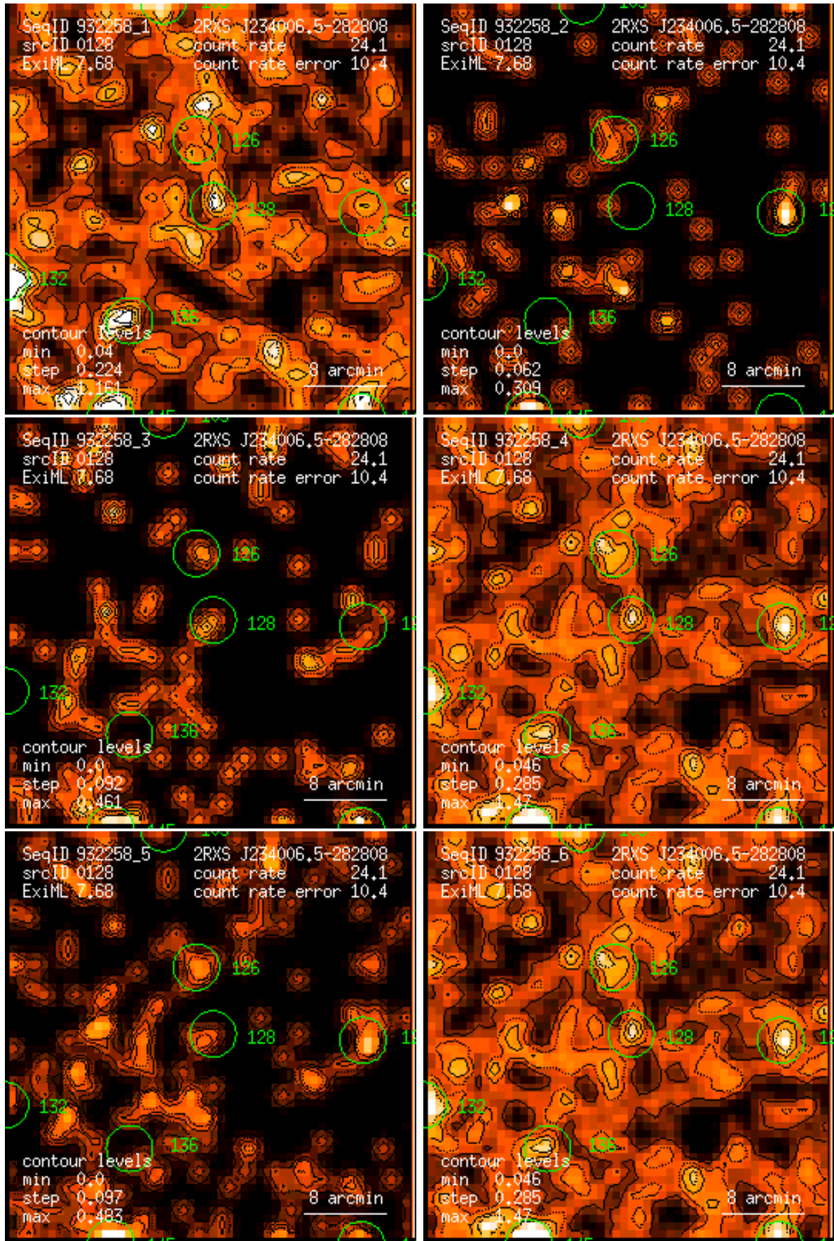
Figure 128: RASS 932258: detection 0128: band rate images, Gaussian filter: (1) PSPC channels 11 – 41, (2) 52 – 90, (3) 91 – 201, (4) 11 – 235, (5) 52 – 201, (6) 11 – 201. Broad band rates in counts/ks. Band rate contour levels in counts/ks/arcmin 2 .
