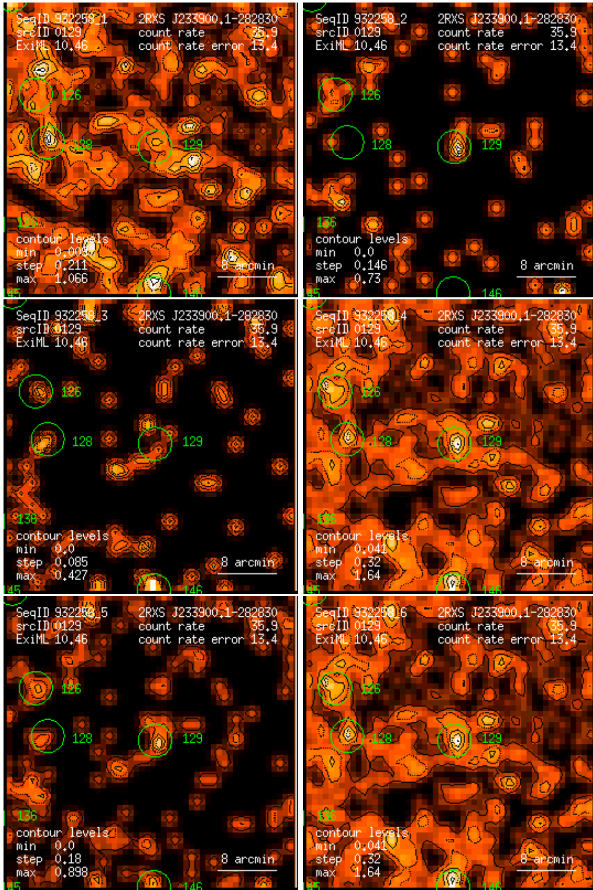
Figure 129: RASS 932258: detection 0129: band rate images, Gaussian filter: (1) PSPC channels 11 – 41, (2) 52 – 90, (3) 91 – 201, (4) 11 – 235, (5) 52 – 201, (6) 11 – 201. Broad band rates in counts/ks. Band rate contour levels in counts/ks/arcmin 2 .
