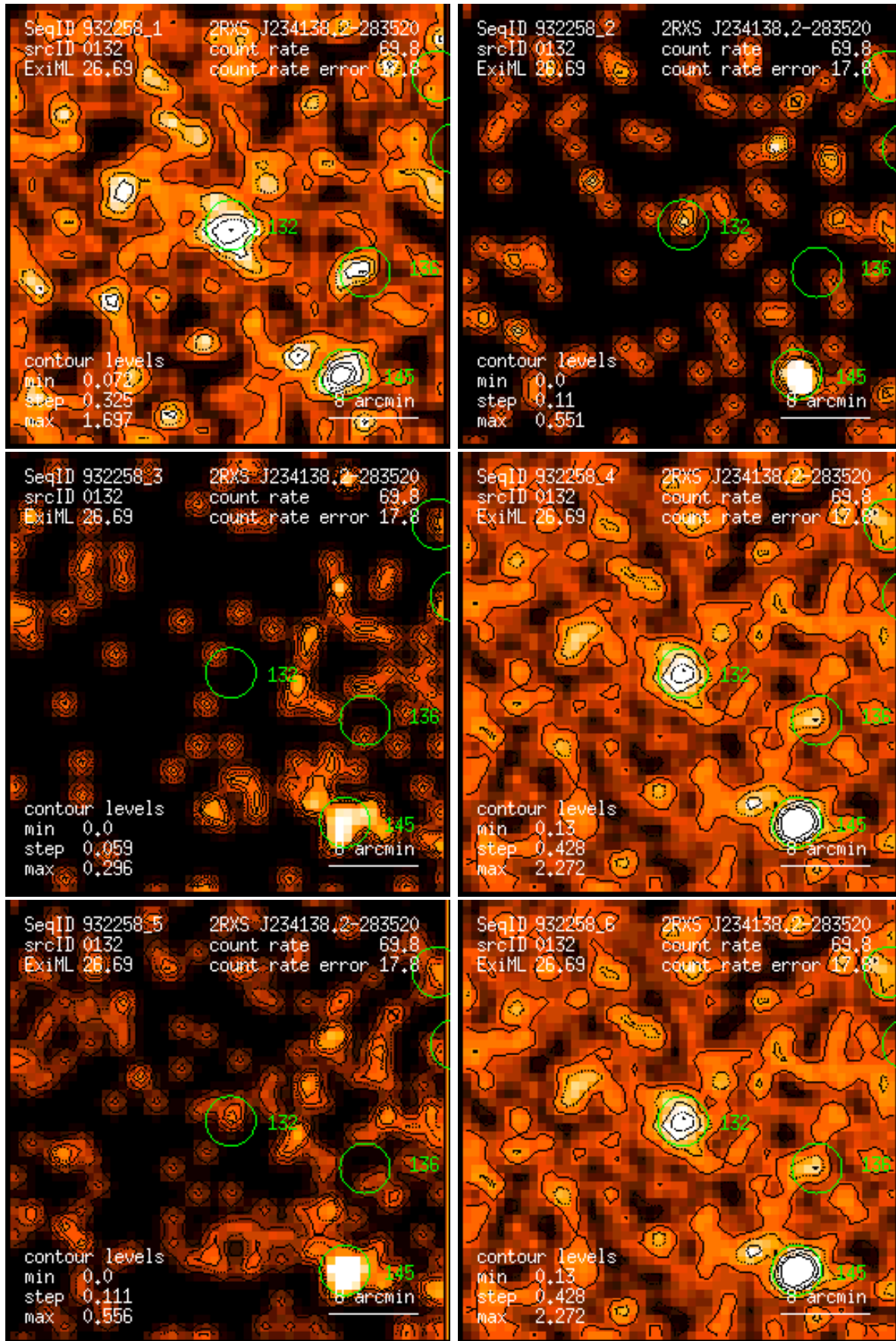
Figure 132: RASS 932258: detection 0132: band rate images, Gaussian filter: (1) PSPC channels 11 – 41, (2) 52 – 90, (3) 91 – 201, (4) 11 – 235, (5) 52 – 201, (6) 11 – 201. Broad band rates in counts/ks. Band rate contour levels in counts/ks/arcmin 2 .
