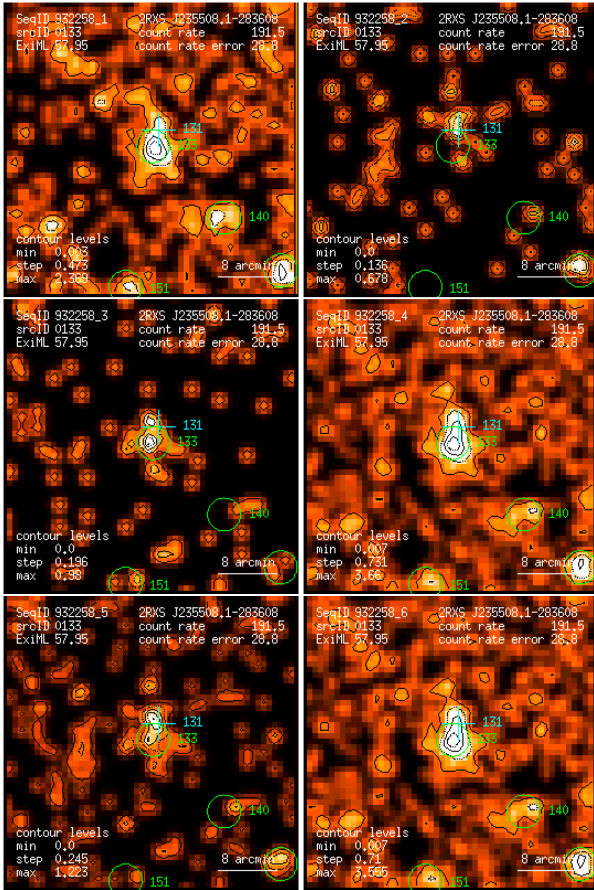
Figure 133: RASS 932258: detection 0133: band rate images, Gaussian filter: (1) PSPC channels 11 – 41, (2) 52 – 90, (3) 91 – 201, (4) 11 – 235, (5) 52 – 201, (6) 11 – 201. Broad band rates in counts/ks. Band rate contour levels in counts/ks/arcmin 2 .
