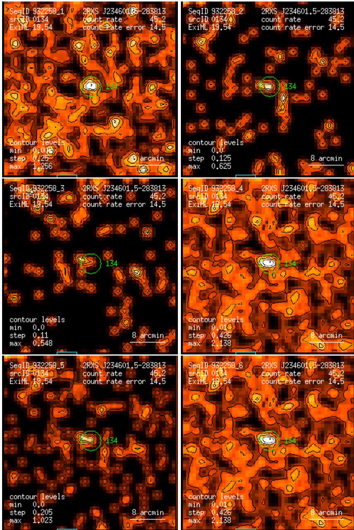
Figure 134: RASS 932258: detection 0134: band rate images, Gaussian filter: (1) PSPC channels 11 – 41, (2) 52 – 90, (3) 91 – 201, (4) 11 – 235, (5) 52 – 201, (6) 11 – 201. Broad band rates in counts/ks. Band rate contour levels in counts/ks/arcmin 2 .
