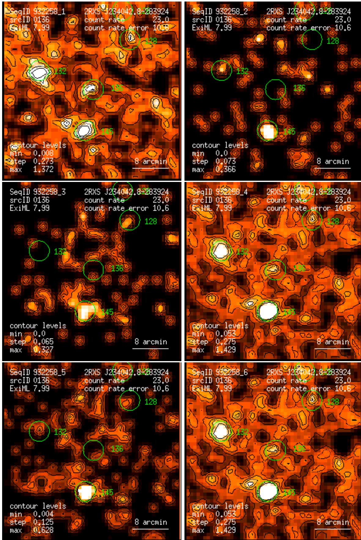
Figure 136: RASS 932258: detection 0136: band rate images, Gaussian filter: (1) PSPC channels 11 – 41, (2) 52 – 90, (3) 91 – 201, (4) 11 – 235, (5) 52 – 201, (6) 11 – 201. Broad band rates in counts/ks. Band rate contour levels in counts/ks/arcmin 2 .
