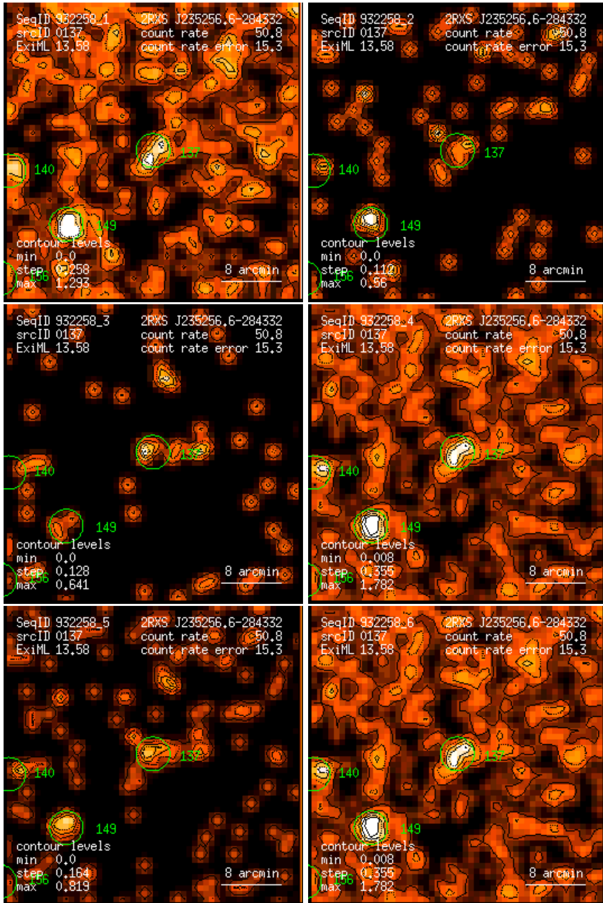
Figure 137: RASS 932258: detection 0137: band rate images, Gaussian filter: (1) PSPC channels 11 – 41, (2) 52 – 90, (3) 91 – 201, (4) 11 – 235, (5) 52 – 201, (6) 11 – 201. Broad band rates in counts/ks. Band rate contour levels in counts/ks/arcmin 2 .
