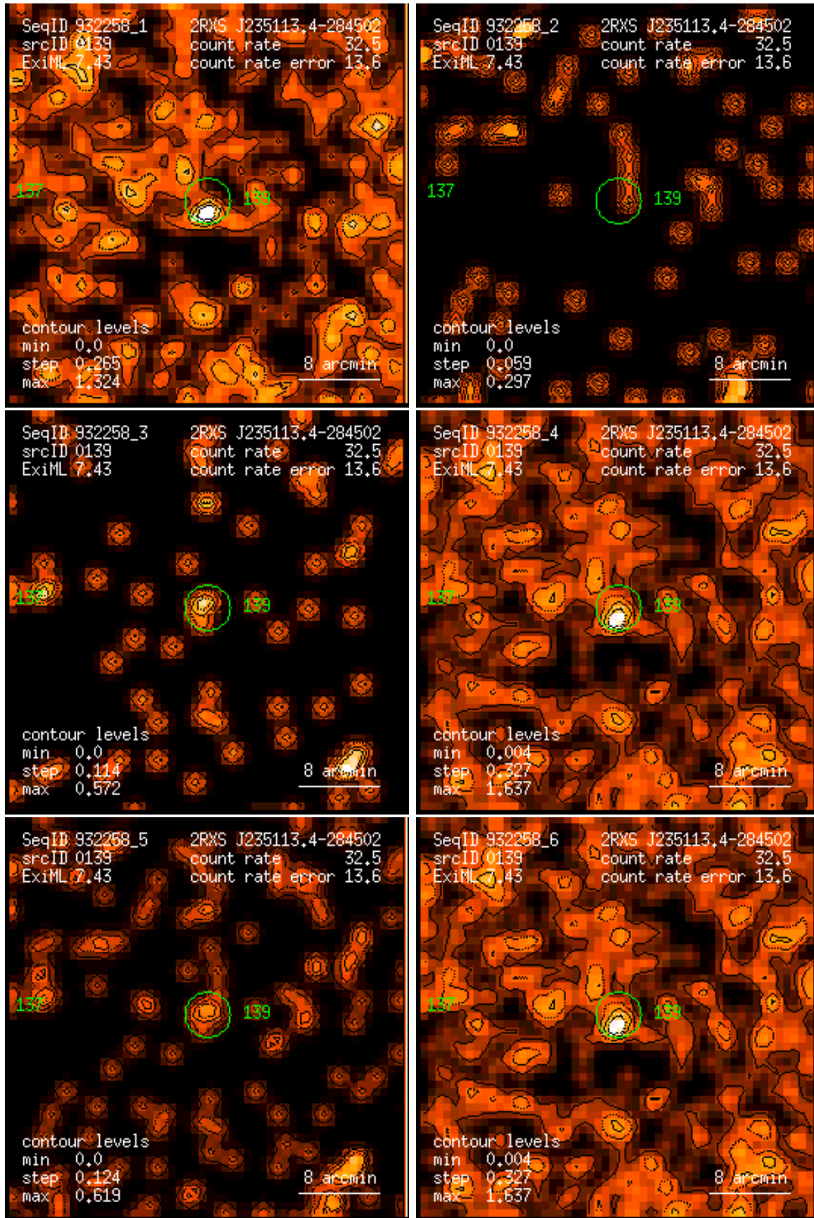
Figure 139: RASS 932258: detection 0139: band rate images, Gaussian filter: (1) PSPC channels 11 – 41, (2) 52 – 90, (3) 91 – 201, (4) 11 – 235, (5) 52 – 201, (6) 11 – 201. Broad band rates in counts/ks. Band rate contour levels in counts/ks/arcmin 2 .
