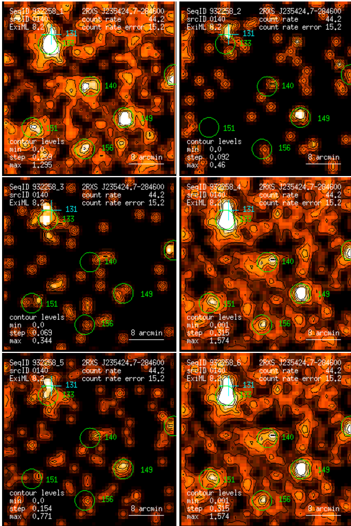
Figure 140: RASS 932258: detection 0140: band rate images, Gaussian filter: (1) PSPC channels 11 – 41, (2) 52 – 90, (3) 91 – 201, (4) 11 – 235, (5) 52 – 201, (6) 11 – 201. Broad band rates in counts/ks. Band rate contour levels in counts/ks/arcmin 2 .
