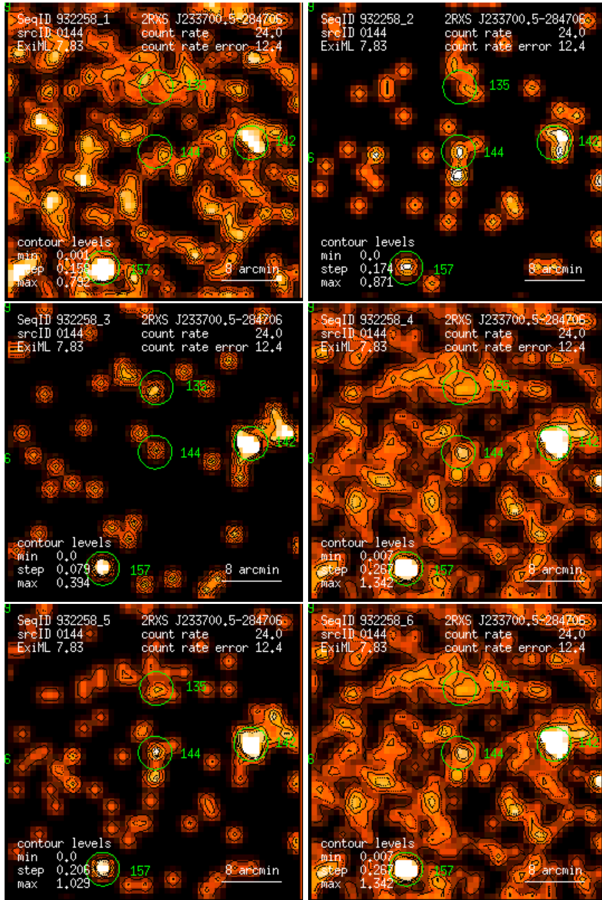
Figure 144: RASS 932258: detection 0144: band rate images, Gaussian filter: (1) PSPC channels 11 – 41, (2) 52 – 90, (3) 91 – 201, (4) 11 – 235, (5) 52 – 201, (6) 11 – 201. Broad band rates in counts/ks. Band rate contour levels in counts/ks/arcmin 2 .
