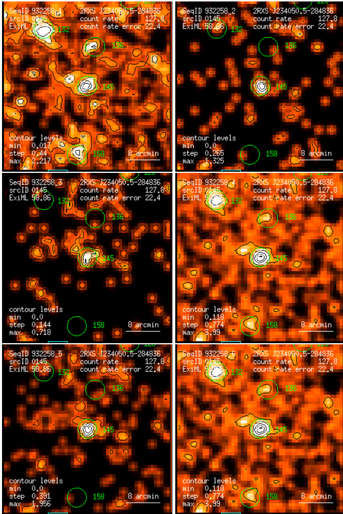
Figure 145: RASS 932258: detection 0145: band rate images, Gaussian filter: (1) PSPC channels 11 – 41, (2) 52 – 90, (3) 91 – 201, (4) 11 – 235, (5) 52 – 201, (6) 11 – 201. Broad band rates in counts/ks. Band rate contour levels in counts/ks/arcmin 2 .
