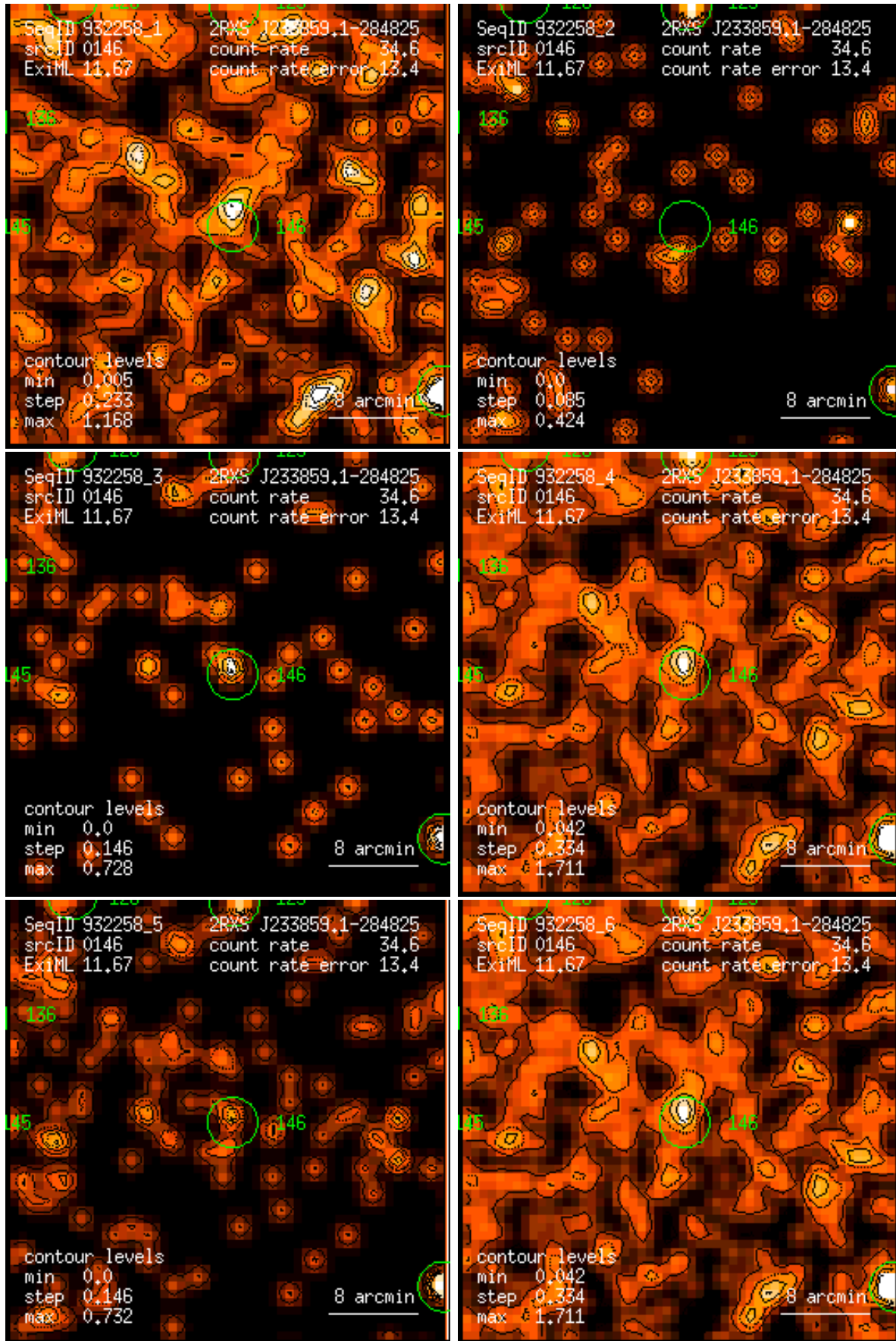
Figure 146: RASS 932258: detection 0146: band rate images, Gaussian filter: (1) PSPC channels 11 – 41, (2) 52 – 90, (3) 91 – 201, (4) 11 – 235, (5) 52 – 201, (6) 11 – 201. Broad band rates in counts/ks. Band rate contour levels in counts/ks/arcmin 2 .
