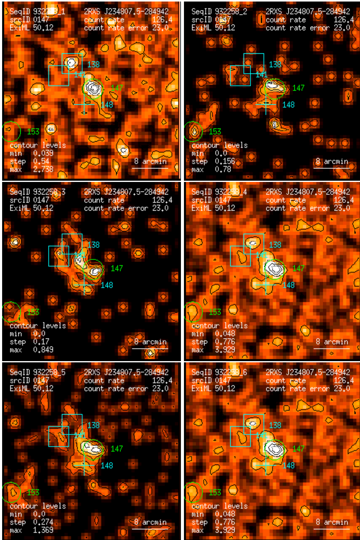
Figure 147: RASS 932258: detection 0147: band rate images, Gaussian filter: (1) PSPC channels 11 – 41, (2) 52 – 90, (3) 91 – 201, (4) 11 – 235, (5) 52 – 201, (6) 11 – 201. Broad band rates in counts/ks. Band rate contour levels in counts/ks/arcmin 2 .
