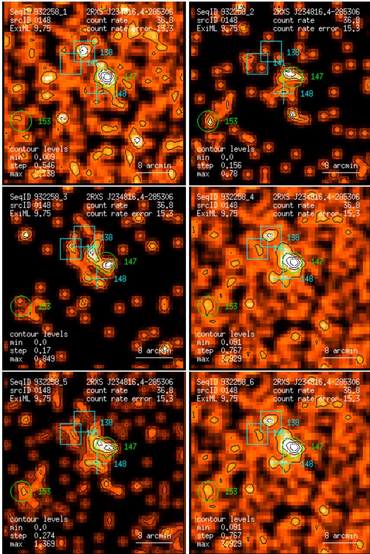
Figure 148: RASS 932258: detection 0148: band rate images, Gaussian filter: (1) PSPC channels 11 – 41, (2) 52 – 90, (3) 91 – 201, (4) 11 – 235, (5) 52 – 201, (6) 11 – 201. Broad band rates in counts/ks. Band rate contour levels in counts/ks/arcmin 2 .
