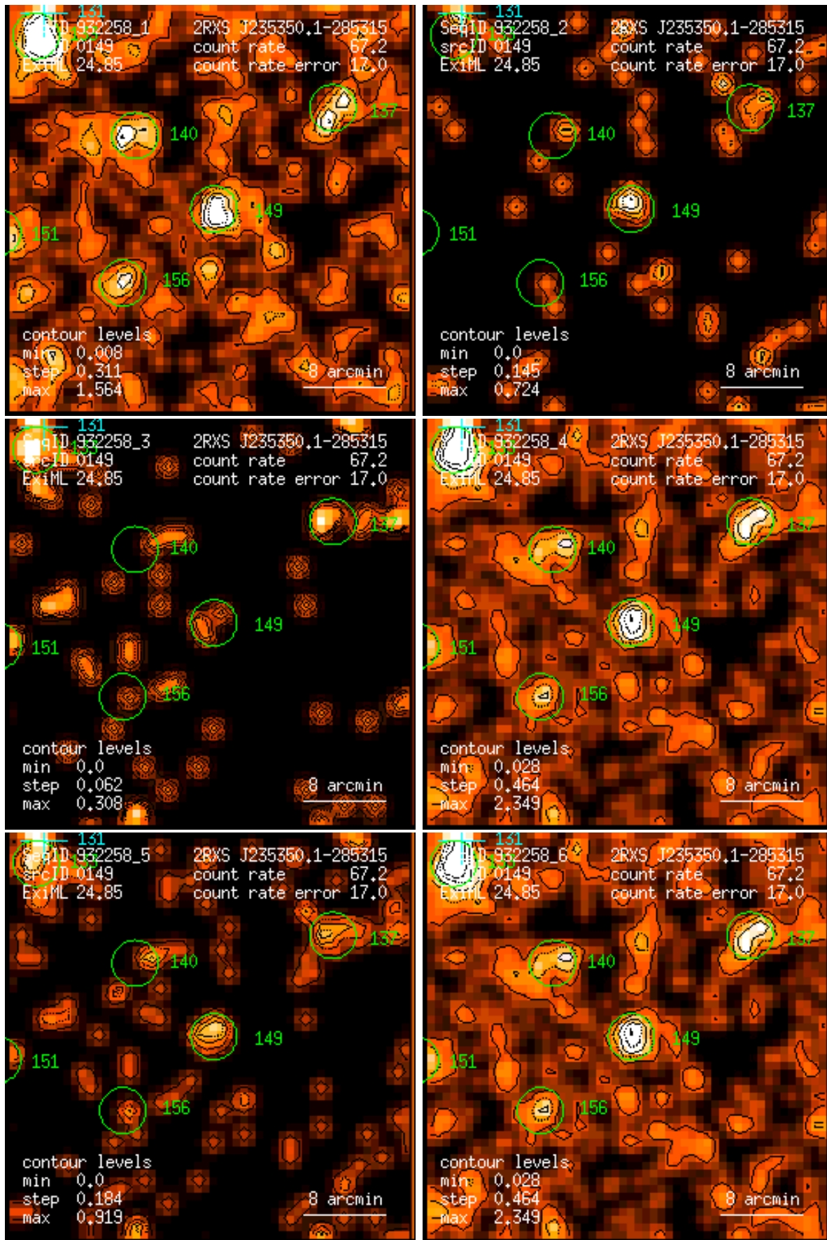
Figure 149: RASS 932258: detection 0149: band rate images, Gaussian filter: (1) PSPC channels 11 – 41, (2) 52 – 90, (3) 91 – 201, (4) 11 – 235, (5) 52 – 201, (6) 11 – 201. Broad band rates in counts/ks. Band rate contour levels in counts/ks/arcmin 2 .
