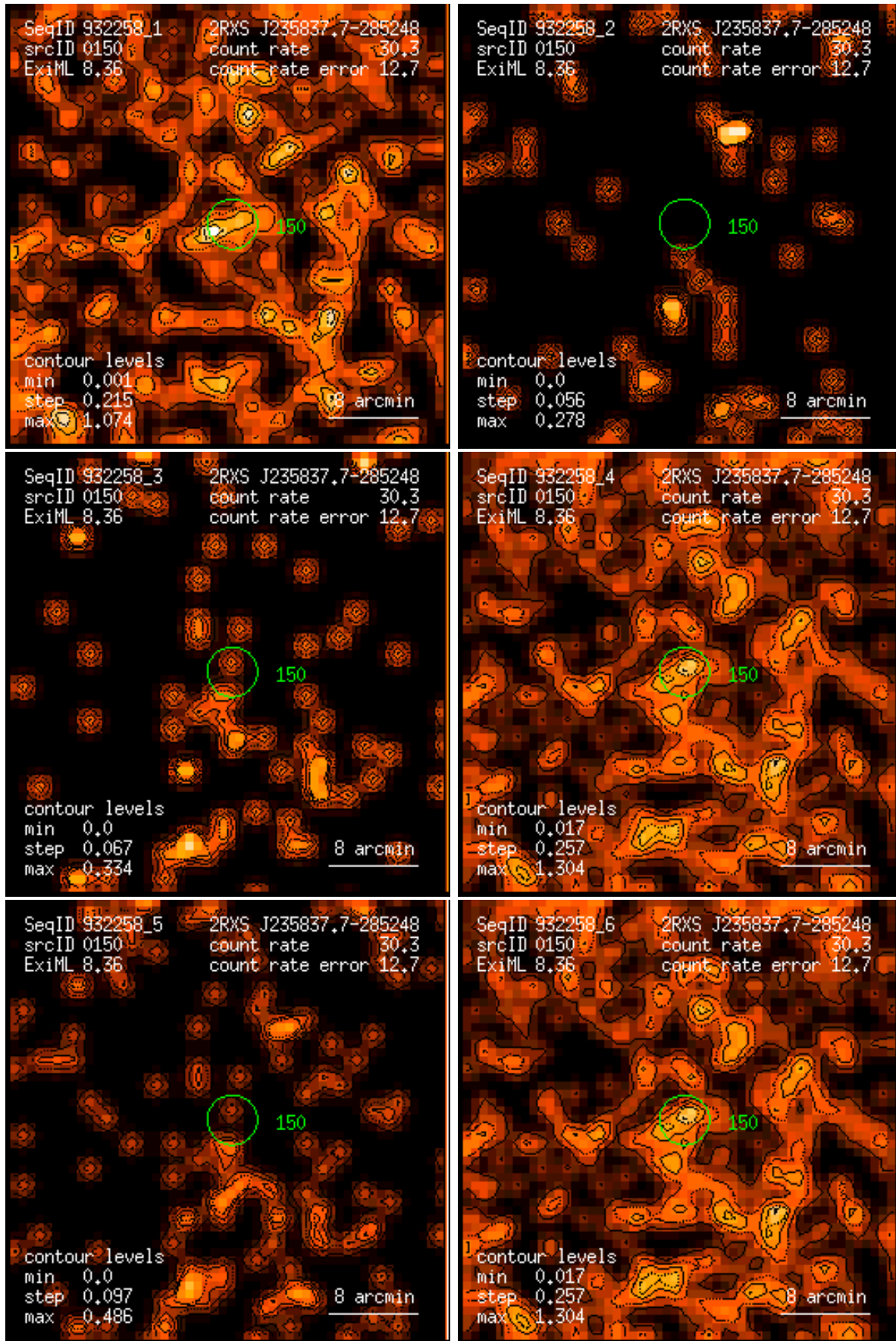
Figure 150: RASS 932258: detection 0150: band rate images, Gaussian filter: (1) PSPC channels 11 – 41, (2) 52 – 90, (3) 91 – 201, (4) 11 – 235, (5) 52 – 201, (6) 11 – 201. Broad band rates in counts/ks. Band rate contour levels in counts/ks/arcmin 2 .
