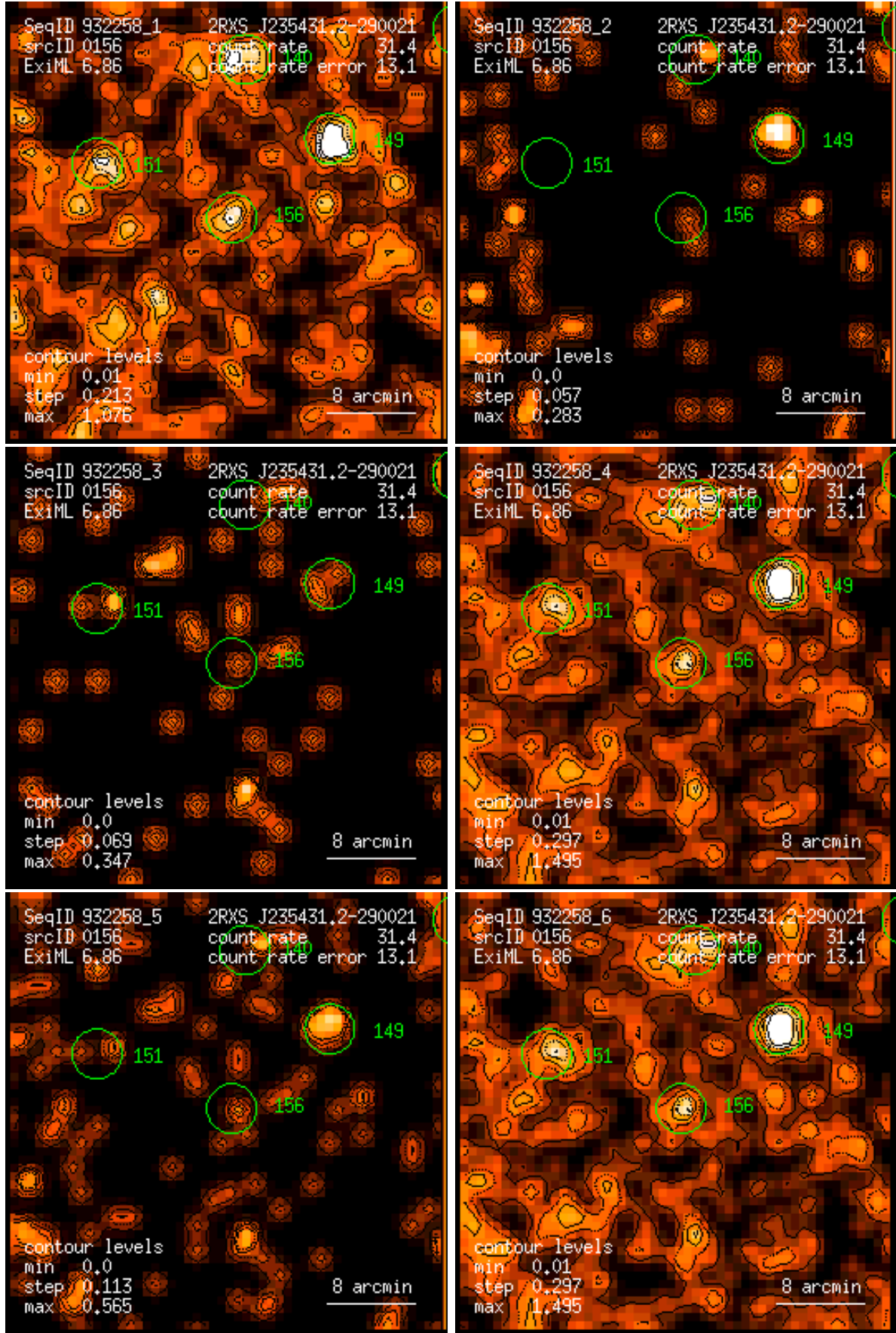
Figure 156: RASS 932258: detection 0156: band rate images, Gaussian filter: (1) PSPC channels 11 – 41, (2) 52 – 90, (3) 91 – 201, (4) 11 – 235, (5) 52 – 201, (6) 11 – 201. Broad band rates in counts/ks. Band rate contour levels in counts/ks/arcmin 2 .
