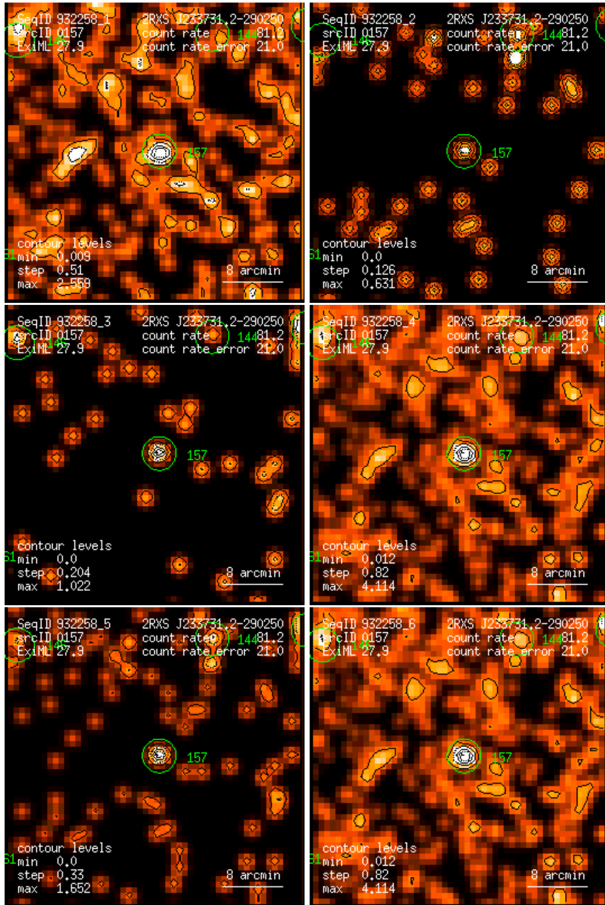
Figure 157: RASS 932258: detection 0157: band rate images, Gaussian filter: (1) PSPC channels 11 – 41, (2) 52 – 90, (3) 91 – 201, (4) 11 – 235, (5) 52 – 201, (6) 11 – 201. Broad band rates in counts/ks. Band rate contour levels in counts/ks/arcmin 2 .
