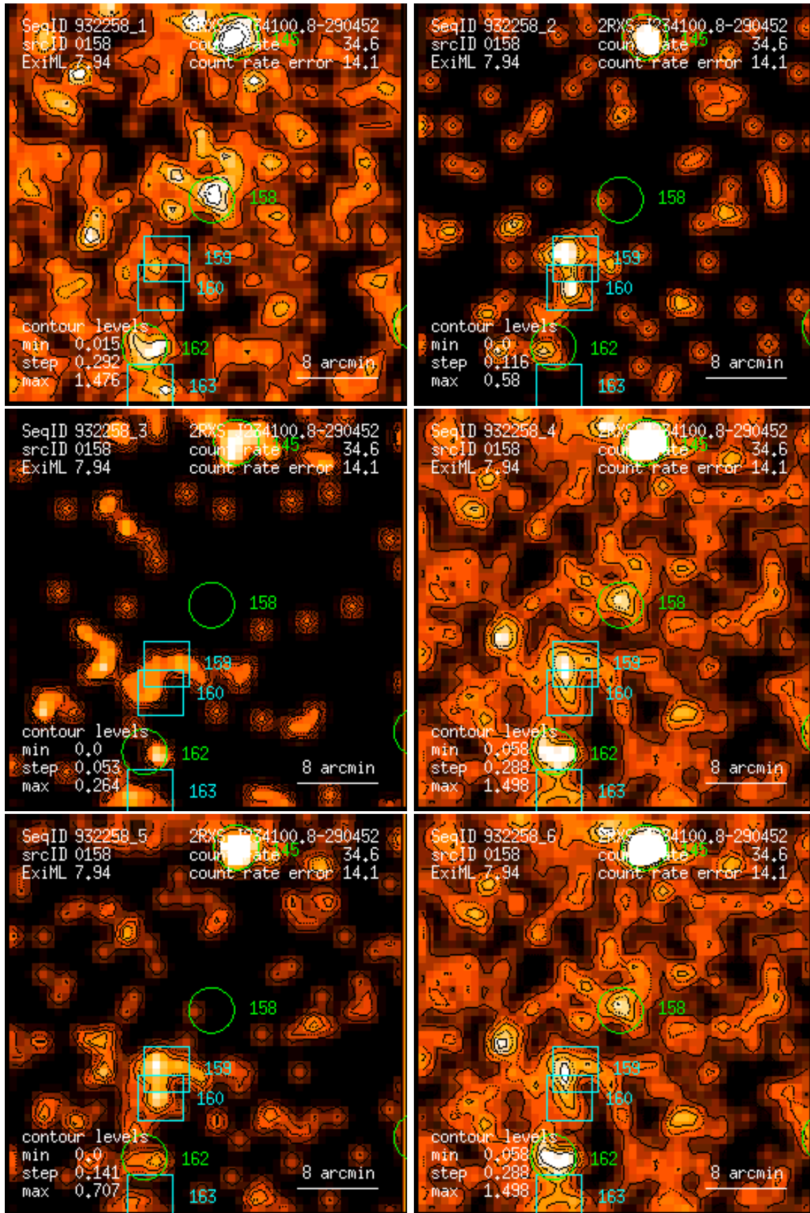
Figure 158: RASS 932258: detection 0158: band rate images, Gaussian filter: (1) PSPC channels 11 – 41, (2) 52 – 90, (3) 91 – 201, (4) 11 – 235, (5) 52 – 201, (6) 11 – 201. Broad band rates in counts/ks. Band rate contour levels in counts/ks/arcmin 2 .
