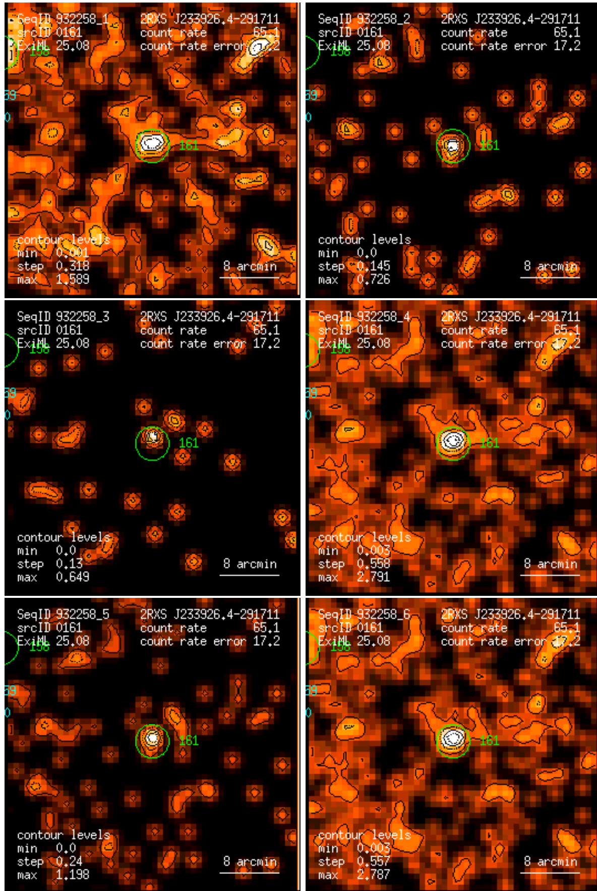
Figure 161: RASS 932258: detection 0161: band rate images, Gaussian filter: (1) PSPC channels 11 – 41, (2) 52 – 90, (3) 91 – 201, (4) 11 – 235, (5) 52 – 201, (6) 11 – 201. Broad band rates in counts/ks. Band rate contour levels in counts/ks/arcmin 2 .
