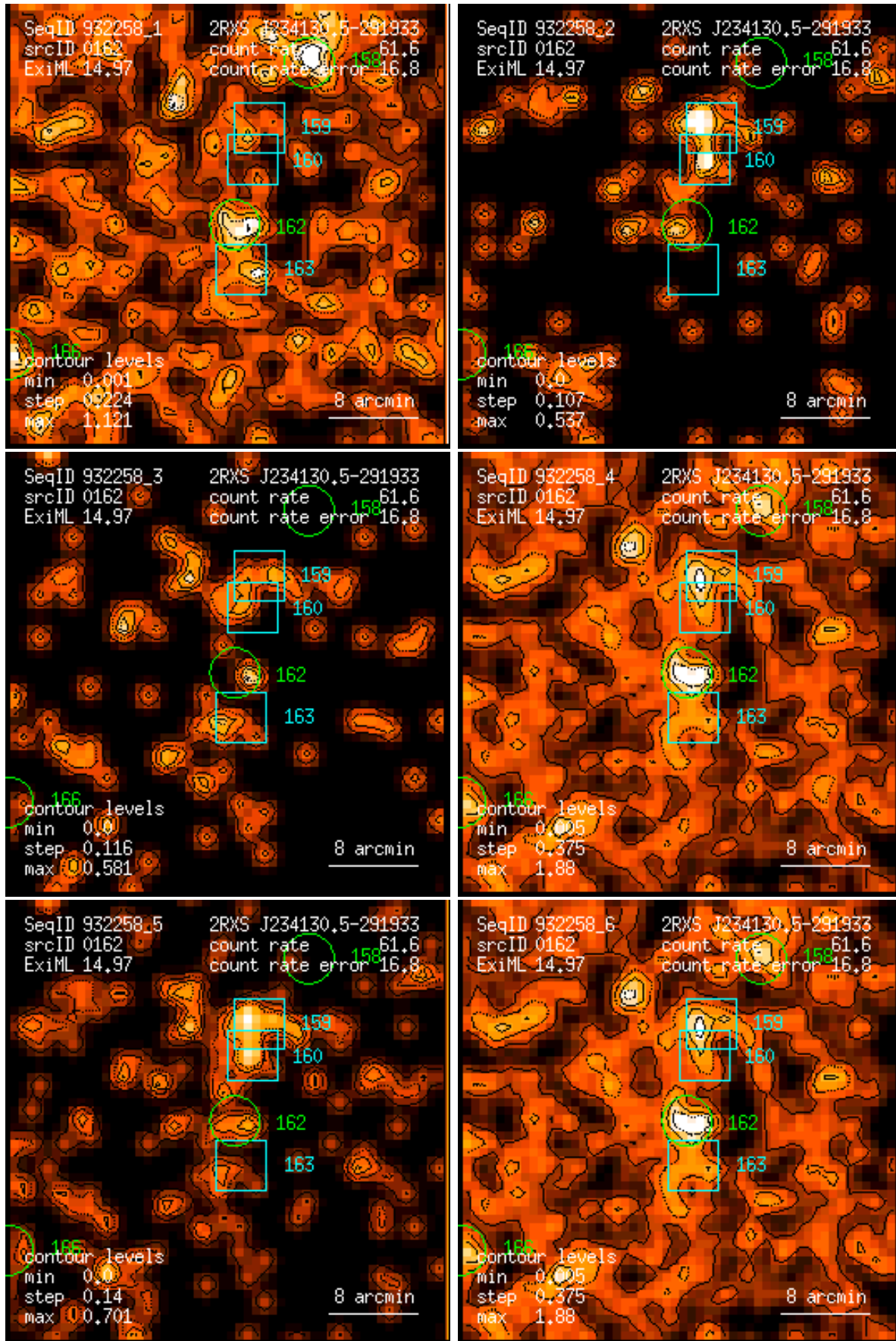
Figure 162: RASS 932258: detection 0162: band rate images, Gaussian filter: (1) PSPC channels 11 – 41, (2) 52 – 90, (3) 91 – 201, (4) 11 – 235, (5) 52 – 201, (6) 11 – 201. Broad band rates in counts/ks. Band rate contour levels in counts/ks/arcmin 2 .
